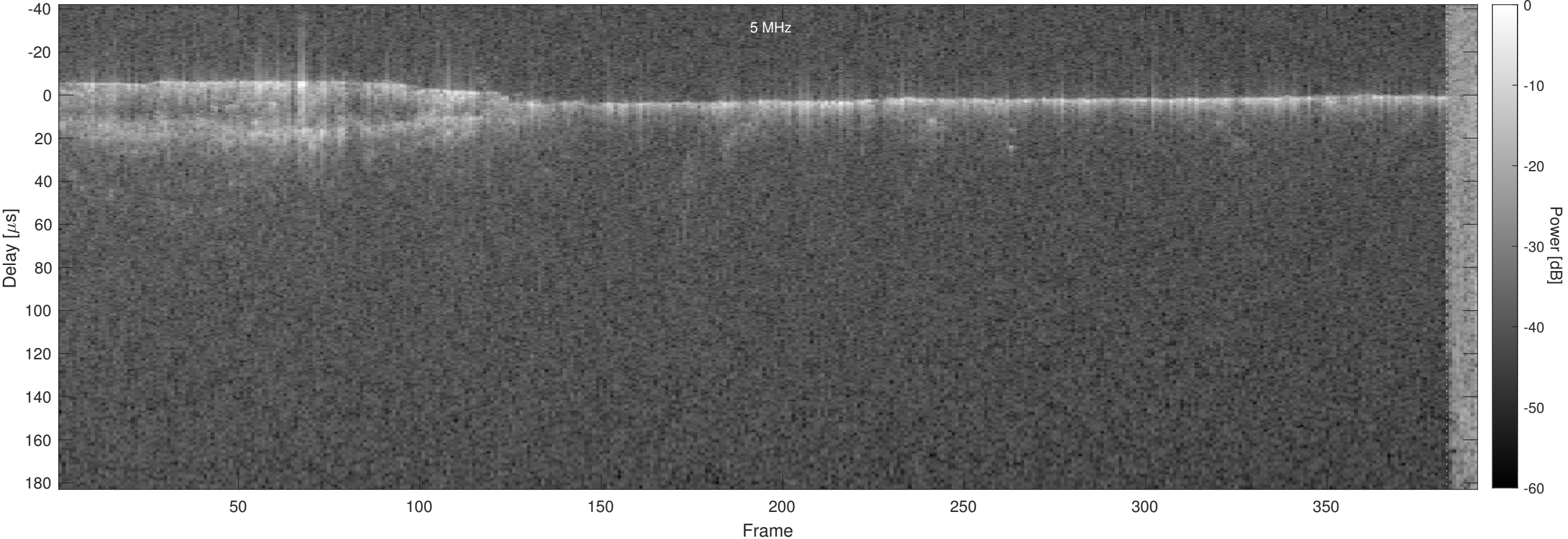
Orbit 5342, Optimized, No Window, Channel 2
