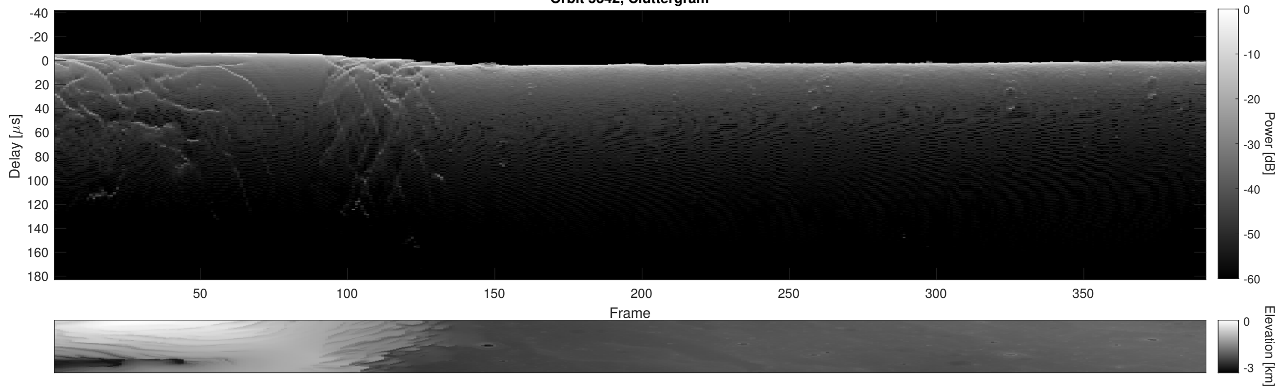
Orbit 5342, Cluttergram
