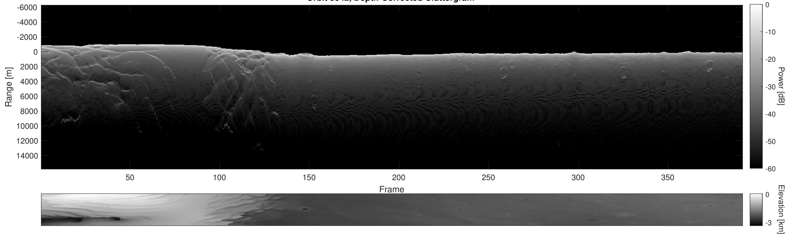
Orbit 5342, Depth-Corrected Cluttergram
