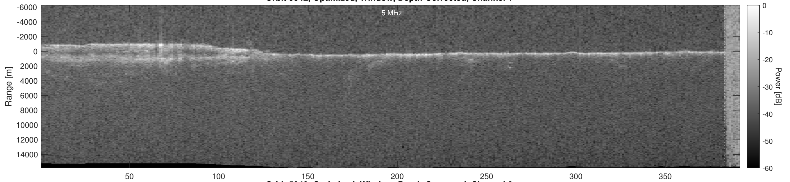
Orbit 5342, Optimized, Window, Depth-Corrected, Channel 2
