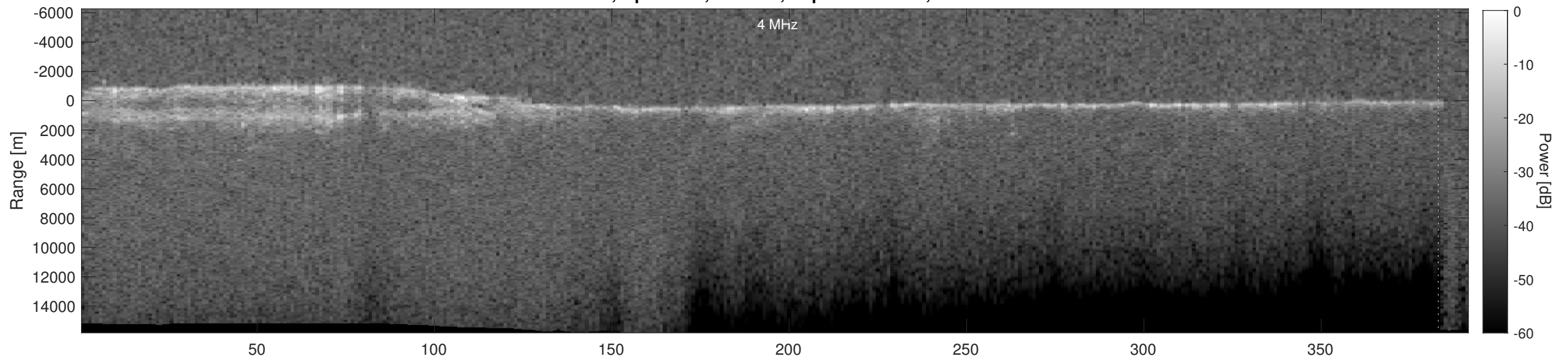
Orbit 5342, Depth-Corrected Cluttergram
