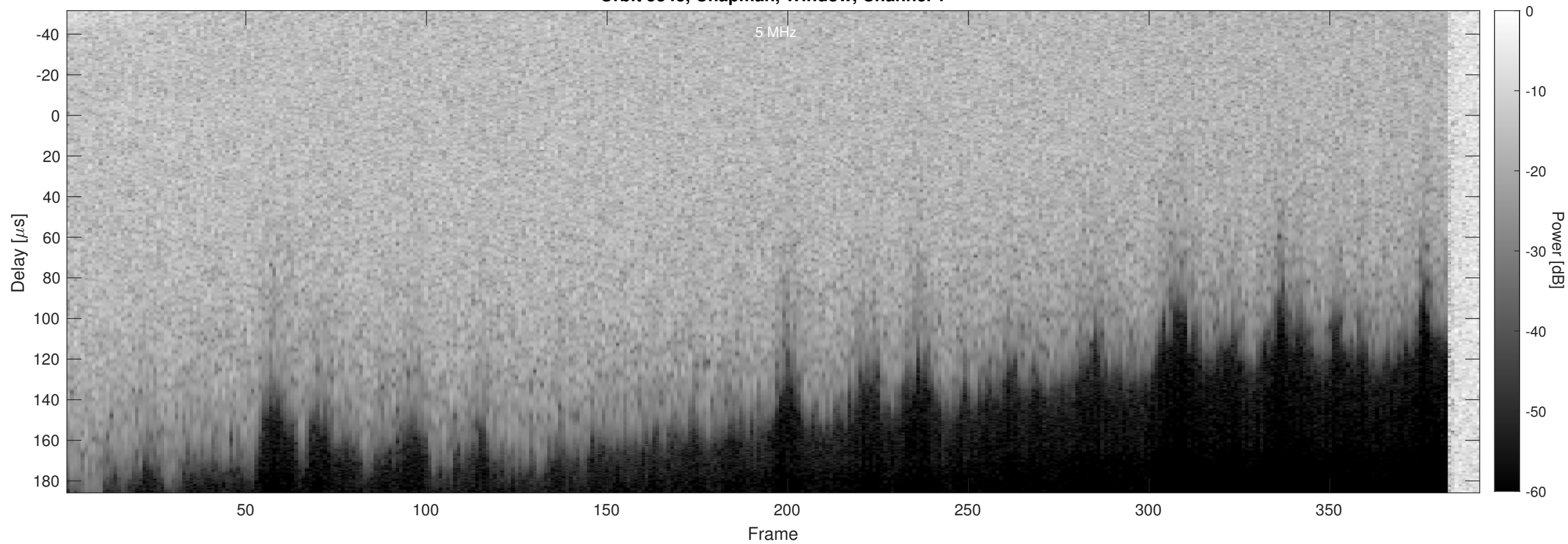
Orbit 5343, Chapman, Window, Channel 2
