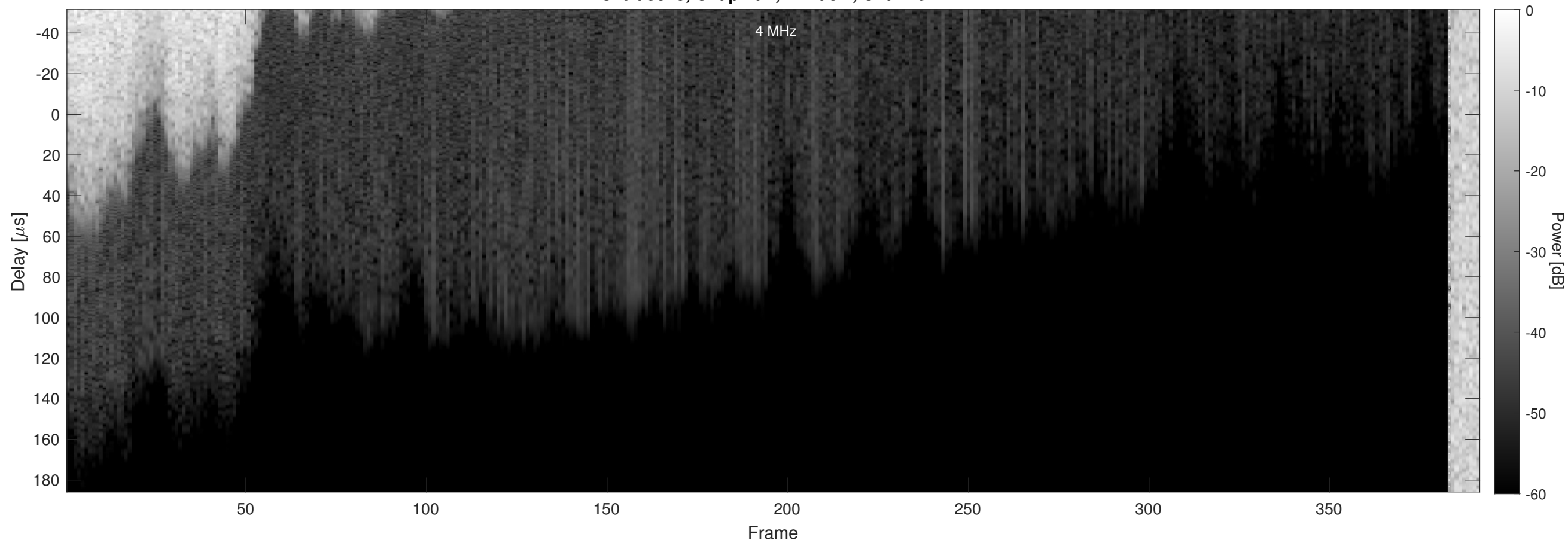
Orbit 5343, Chapman, Window, Channel 2
