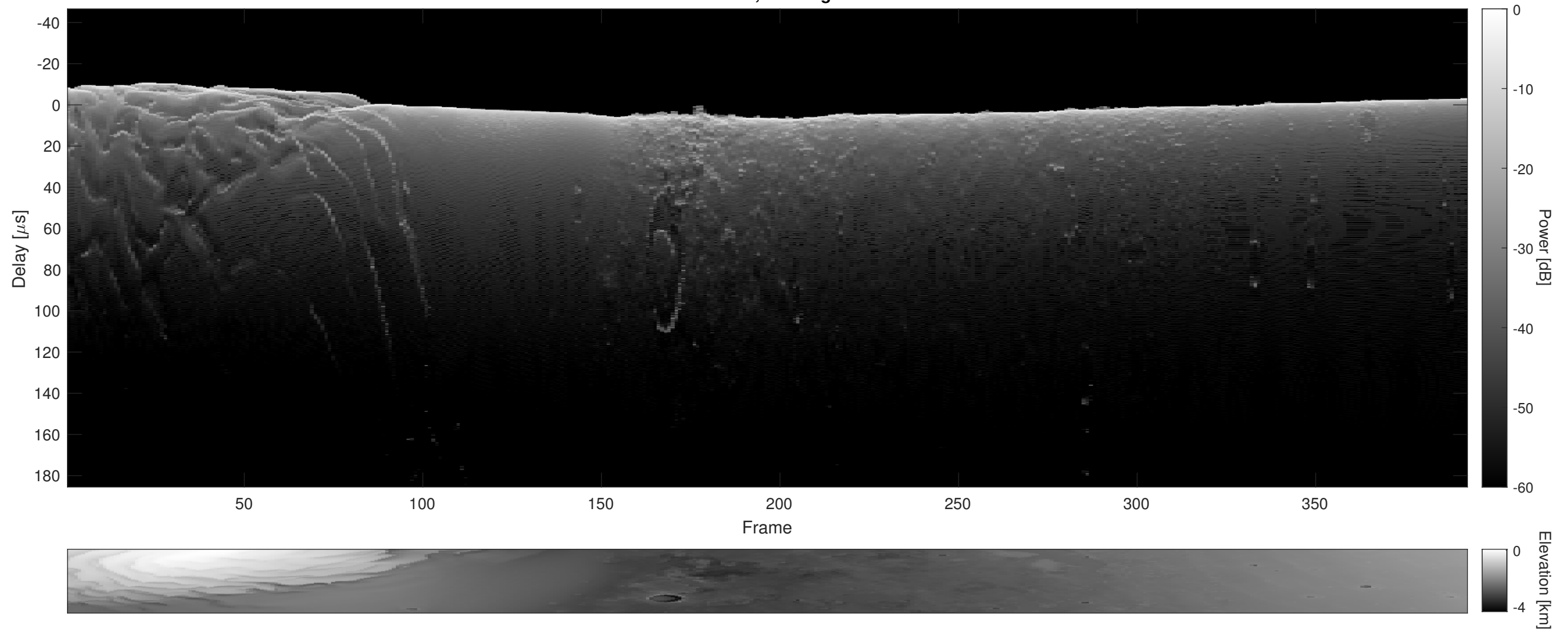
Orbit 5344, Cluttergram
