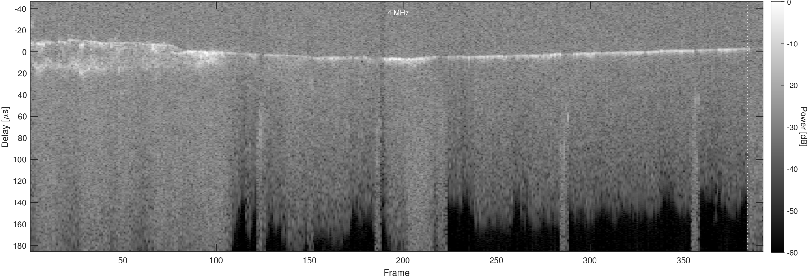
Orbit 5344, Optimized, No Window, Channel 2
