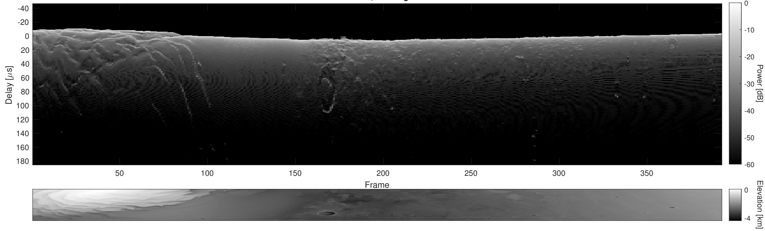
Orbit 5344, Cluttergram
