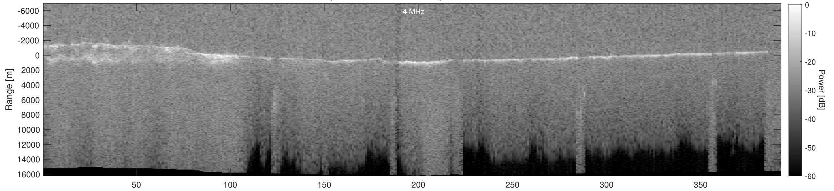
Orbit 5344, Depth-Corrected Cluttergram
