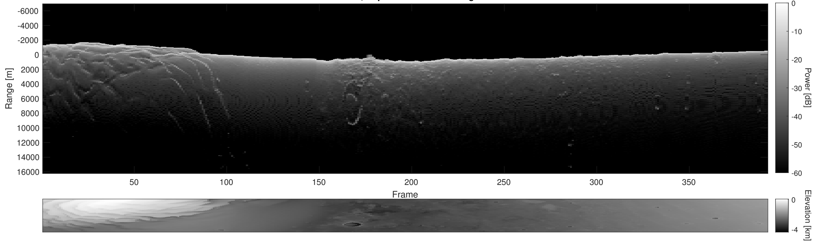
Orbit 5344, Depth-Corrected Cluttergram
