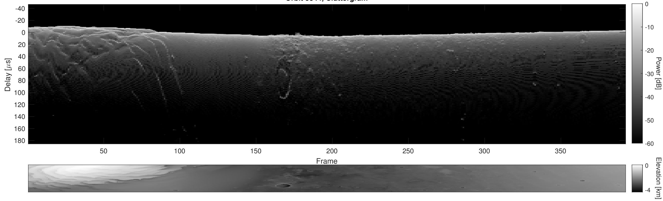
Orbit 5344, Cluttergram
