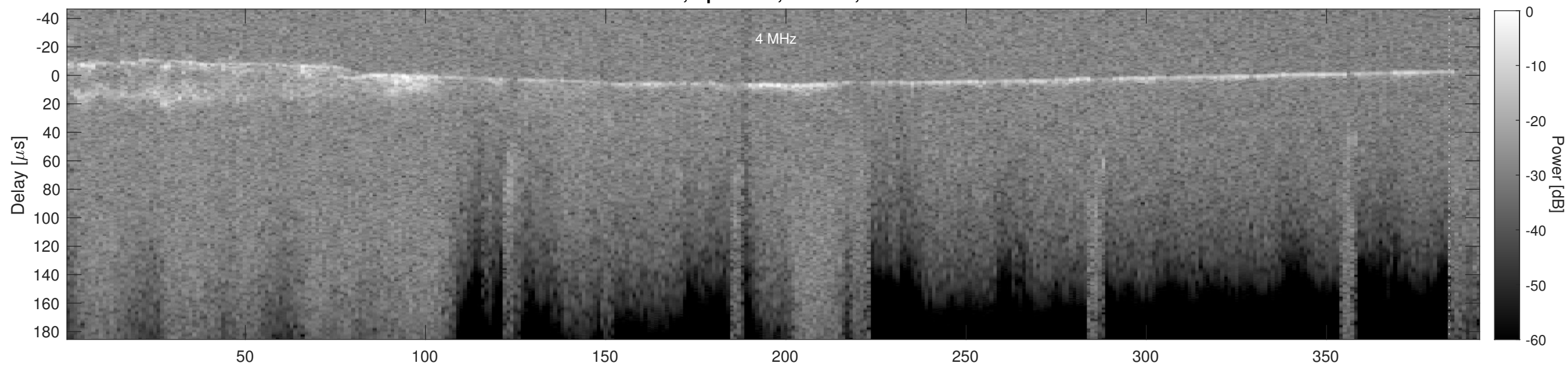
Orbit 5344, Cluttergram
