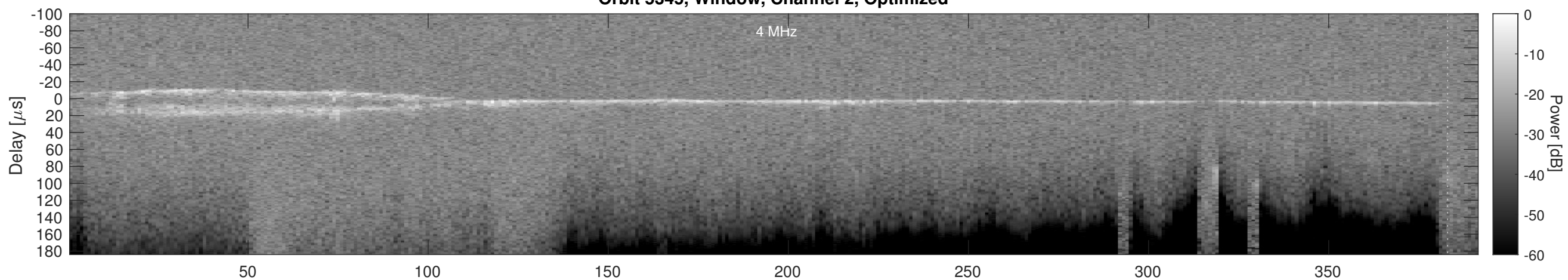
Orbit 5345, Cluttergram
