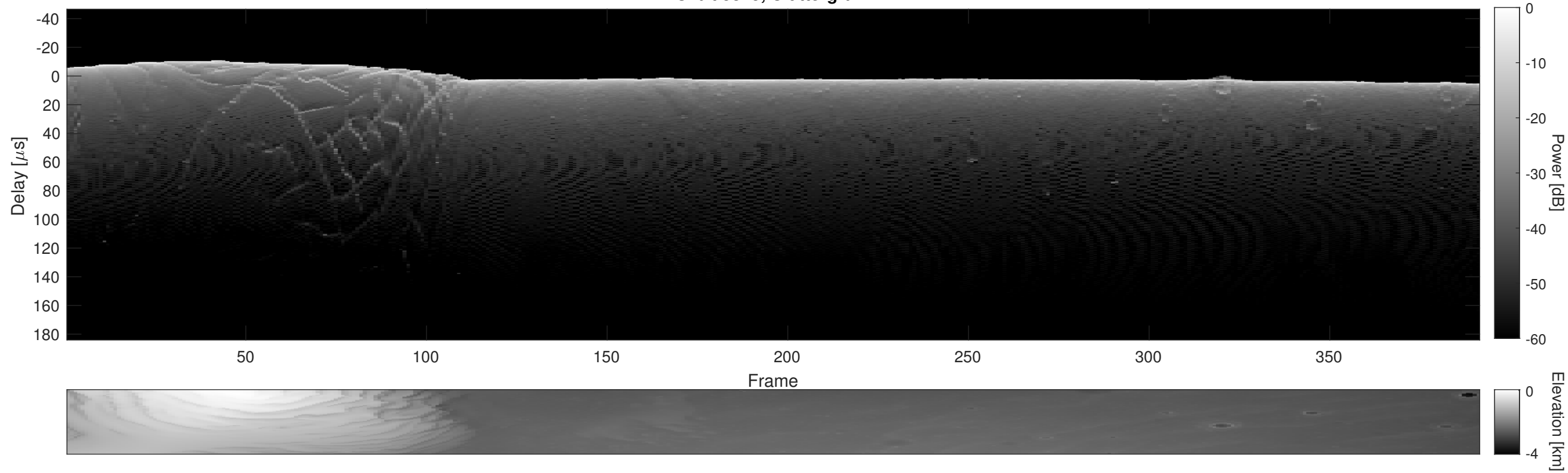
Orbit 5345, Cluttergram
