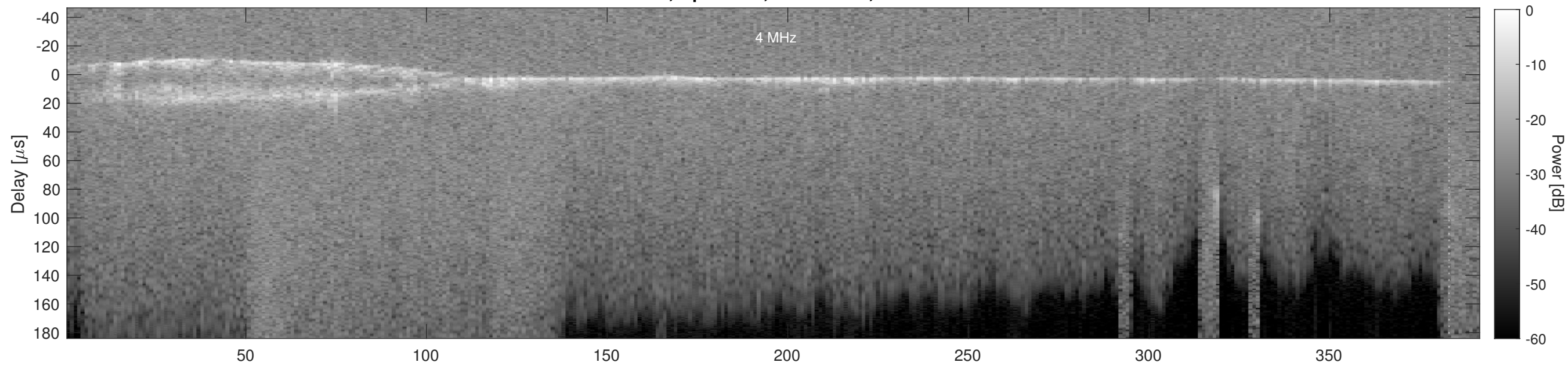
Orbit 5345, Cluttergram
