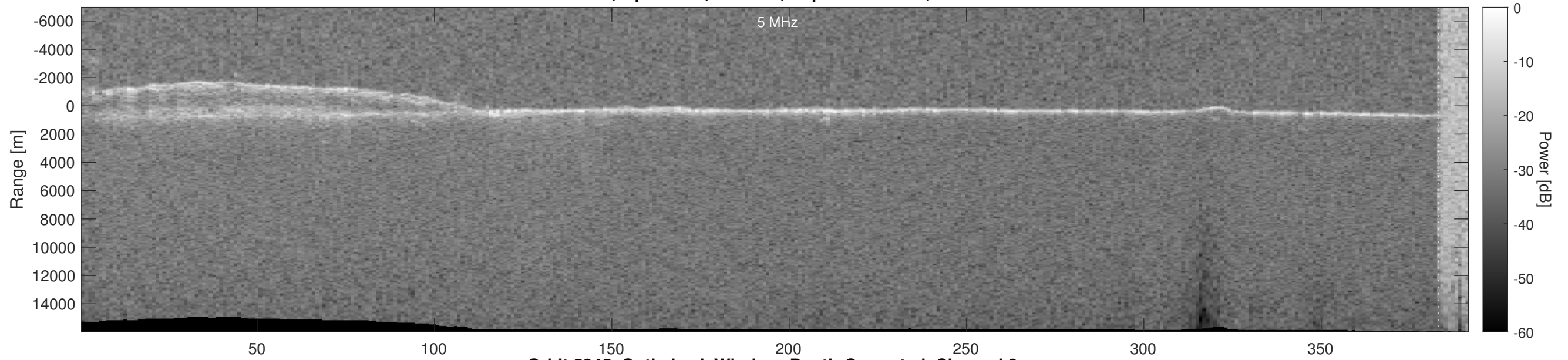
Orbit 5345, Optimized, Window, Depth-Corrected, Channel 2
