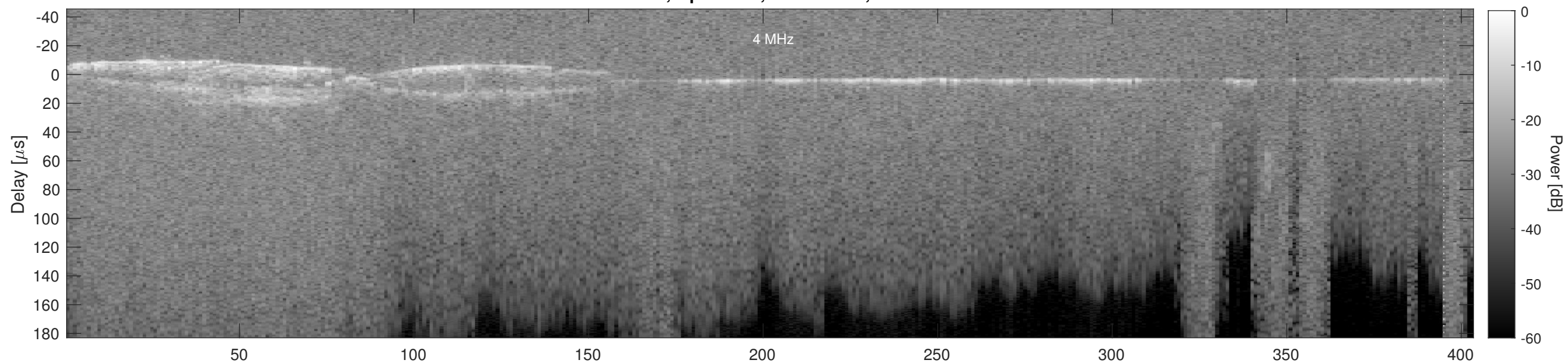
Orbit 5346, Cluttergram
