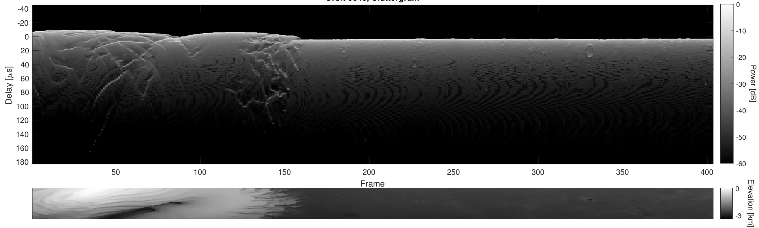
Orbit 5346, Cluttergram
