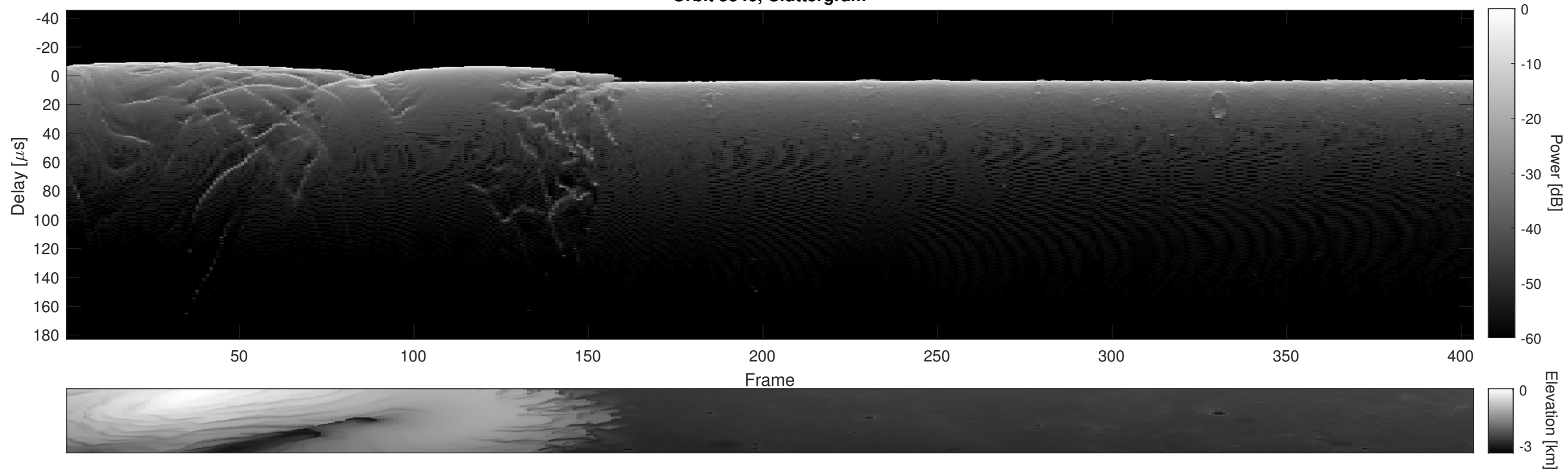
Orbit 5346, Cluttergram
