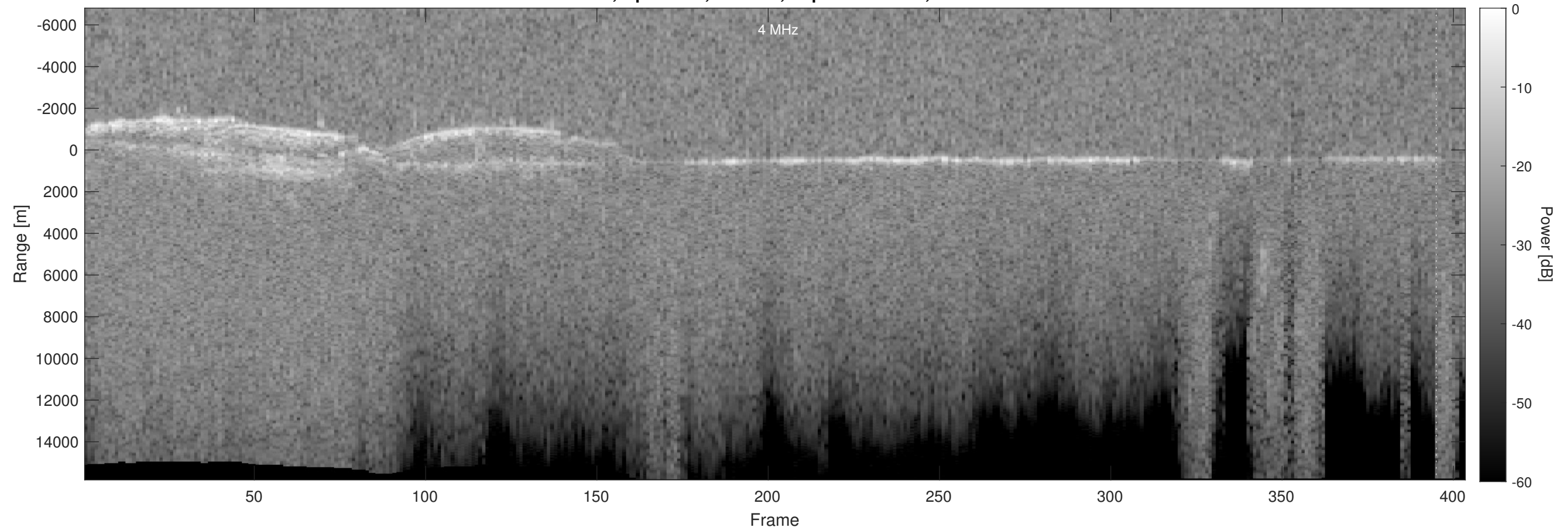
Orbit 5346, Optimized, Window, Depth-Corrected, Channel 2
