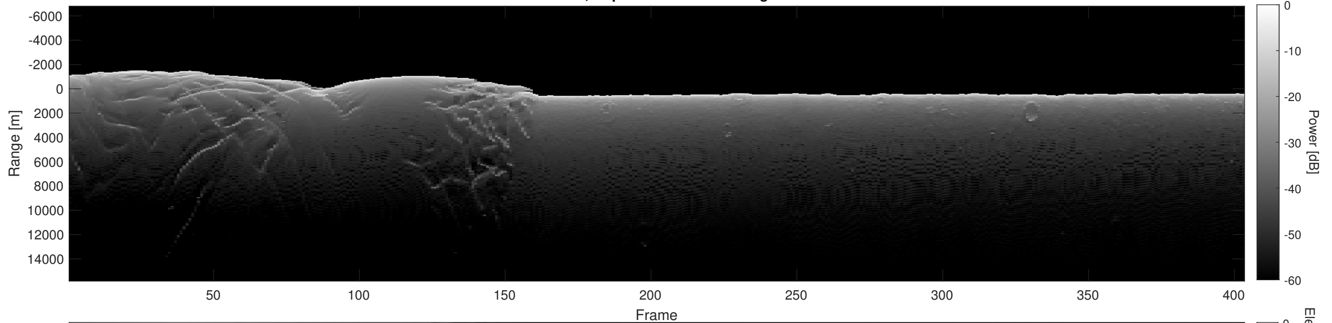
Orbit 5346, Depth-Corrected Cluttergram
