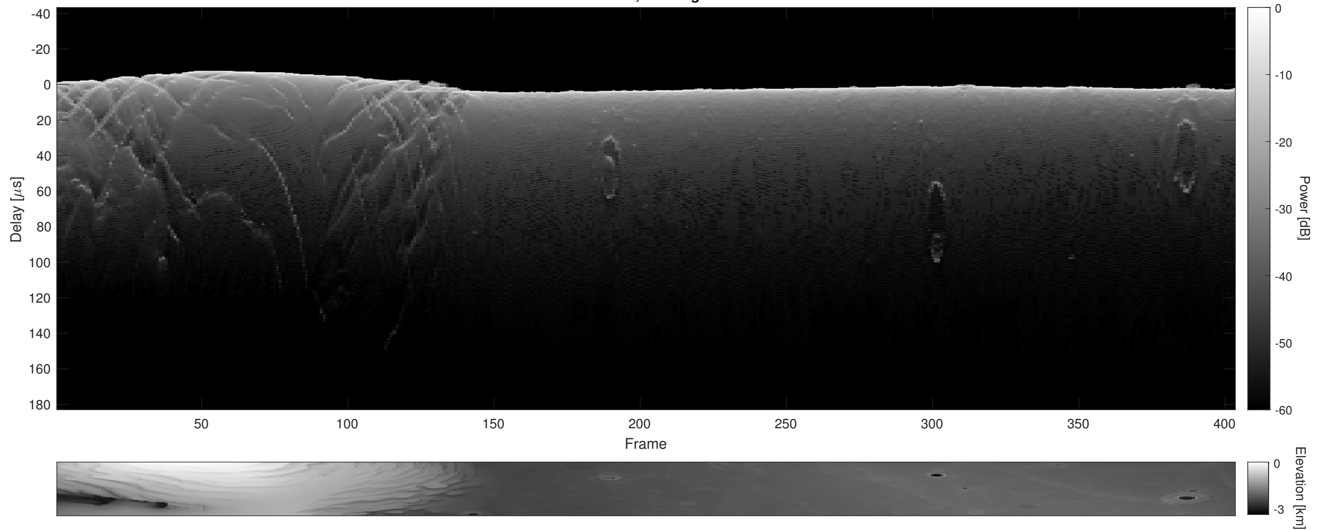
Orbit 5349, Cluttergram
