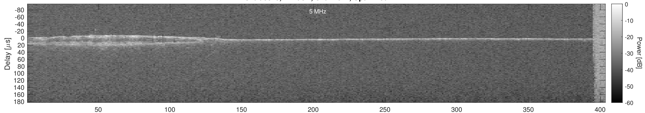
Orbit 5349, Cluttergram
