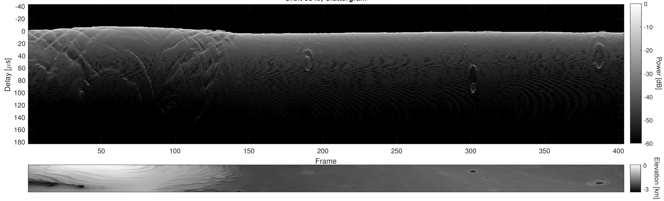
Orbit 5349, Cluttergram
