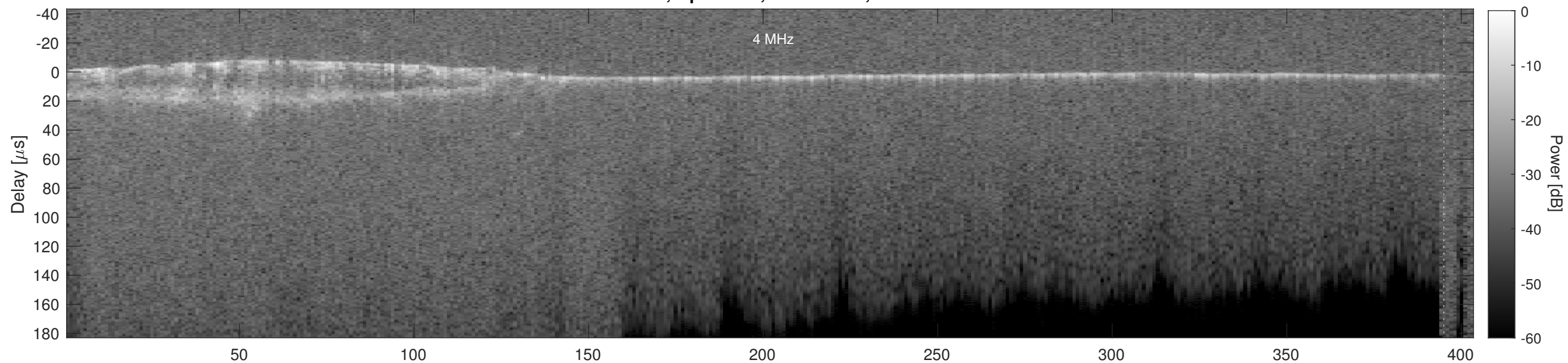
Orbit 5349, Cluttergram
