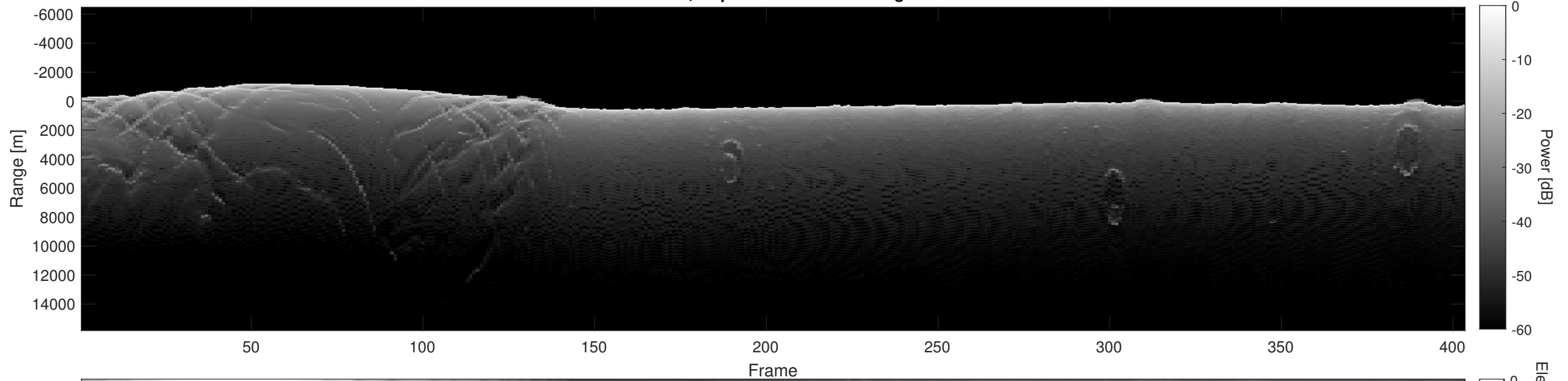
Orbit 5349, Depth-Corrected Cluttergram
