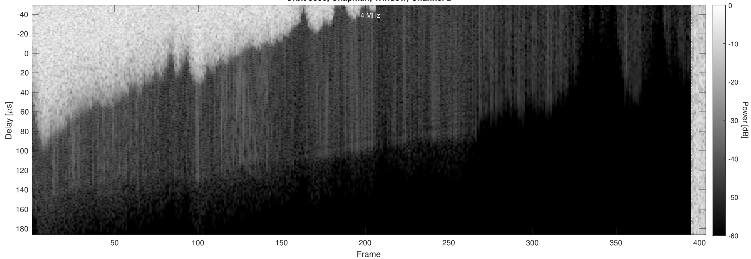
Orbit 5350, Chapman, Window, Channel 2
