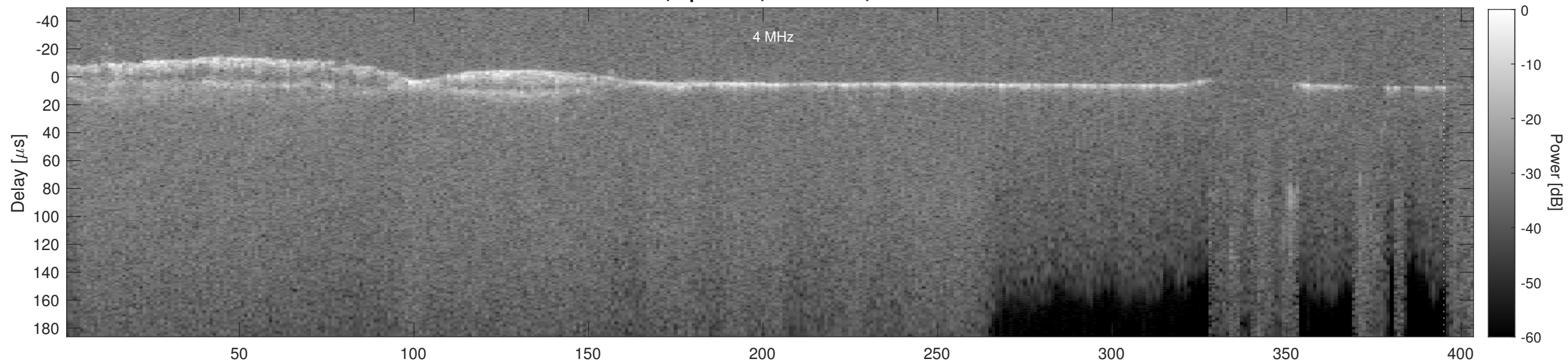
Orbit 5350, Cluttergram
