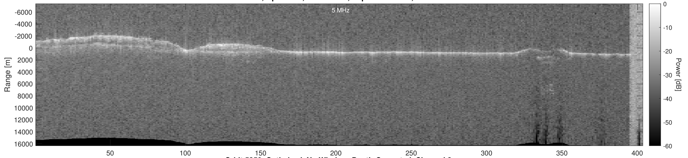
Orbit 5350, Optimized, No Window, Depth-Corrected, Channel 2
