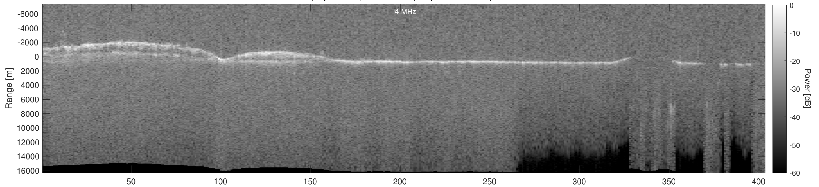
Orbit 5350, Depth-Corrected Cluttergram
