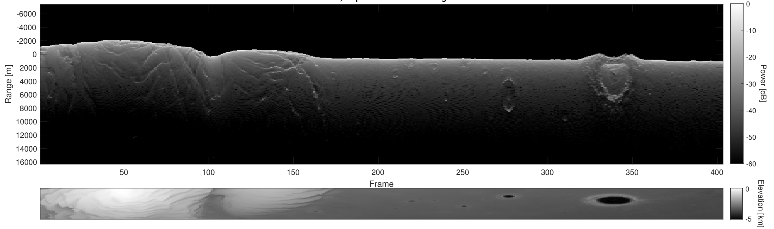
Orbit 5350, Depth-Corrected Cluttergram
