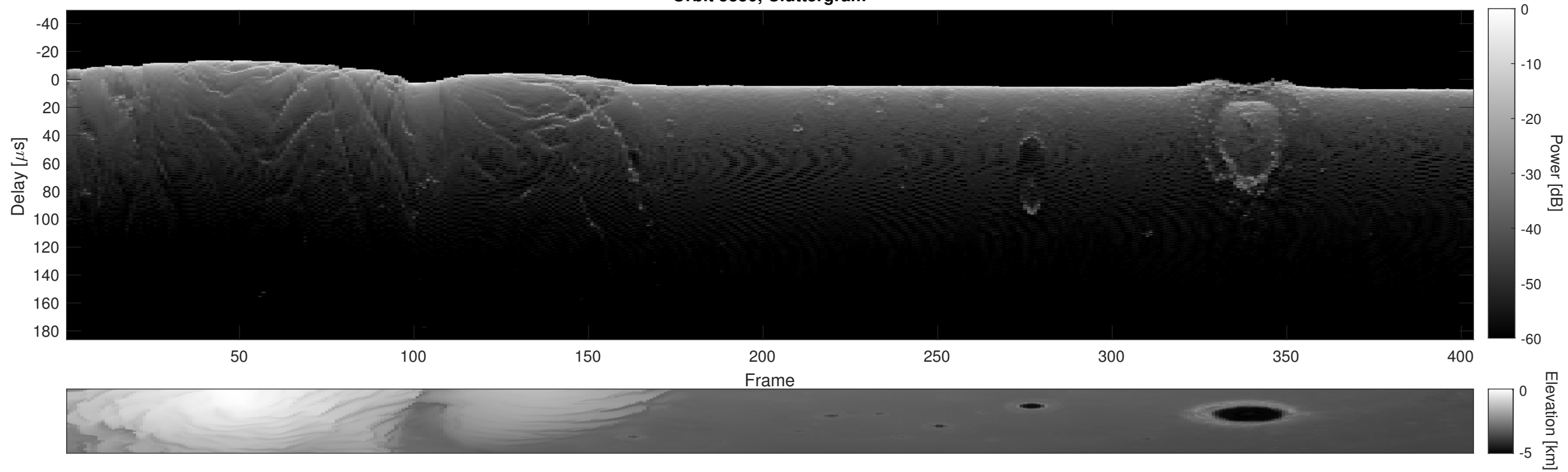
Orbit 5350, Cluttergram
