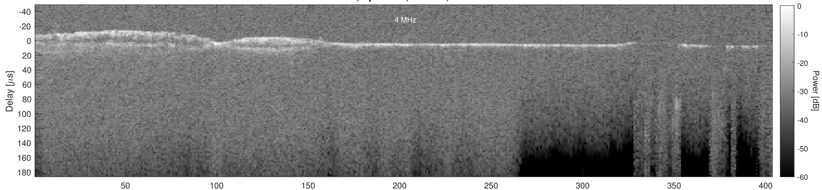
Orbit 5350, Cluttergram
