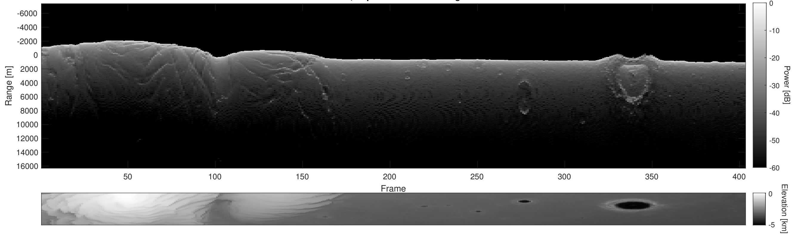
Orbit 5350, Depth-Corrected Cluttergram
