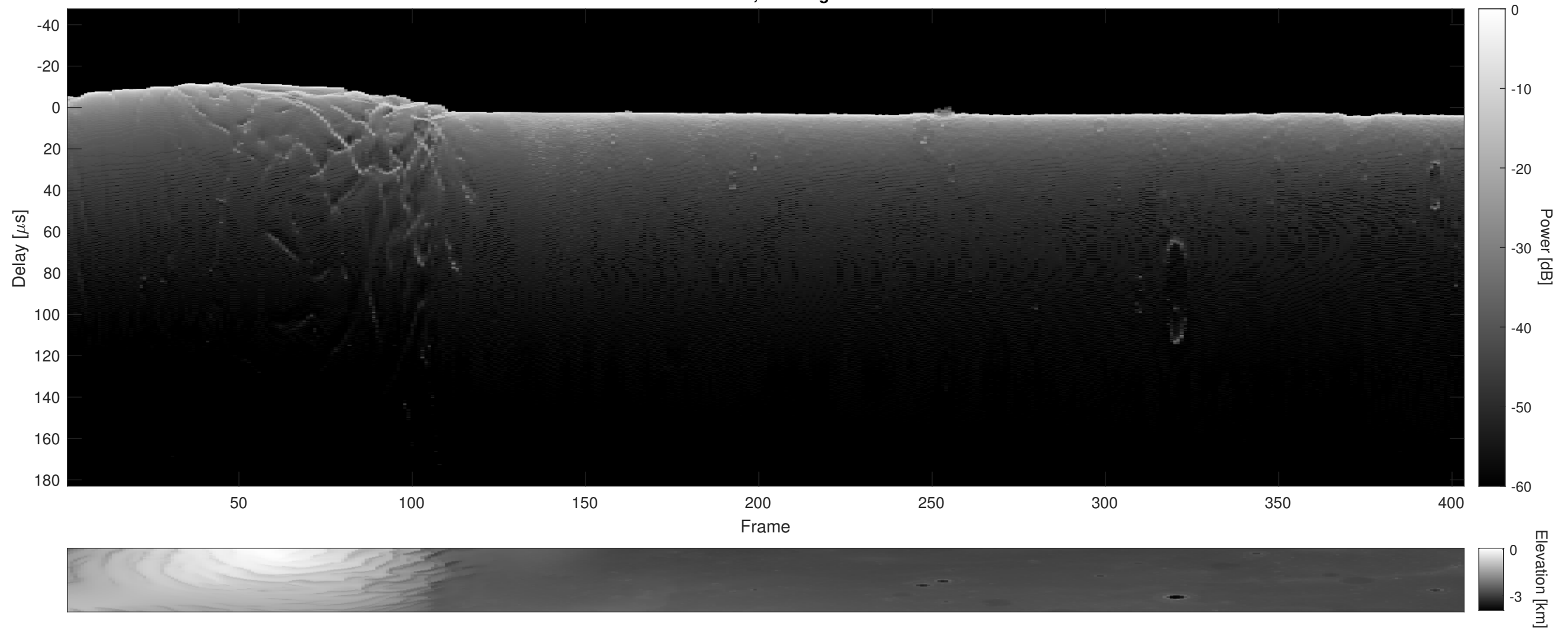
Orbit 5352, Cluttergram
