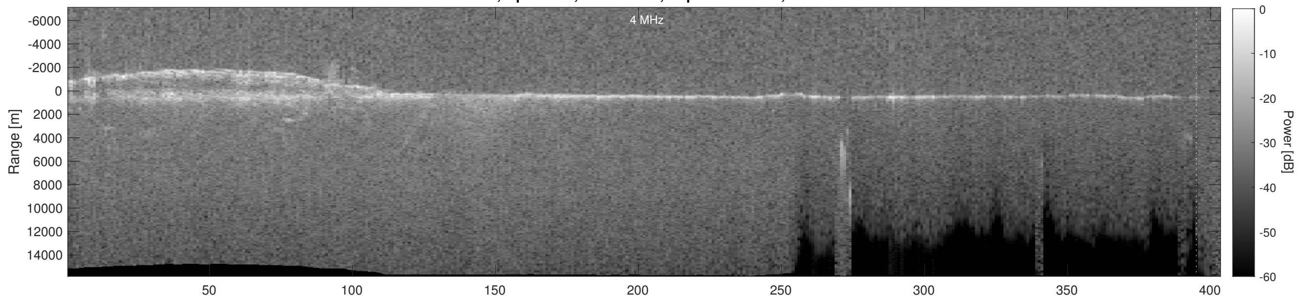
Orbit 5352, Depth-Corrected Cluttergram
