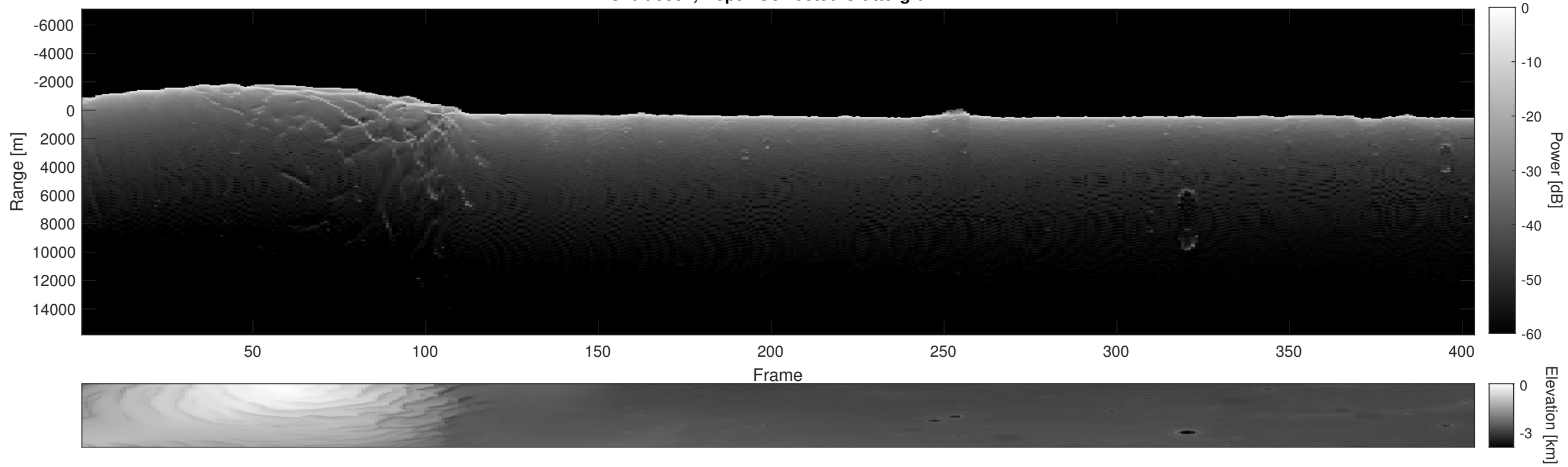
Orbit 5352, Depth-Corrected Cluttergram
