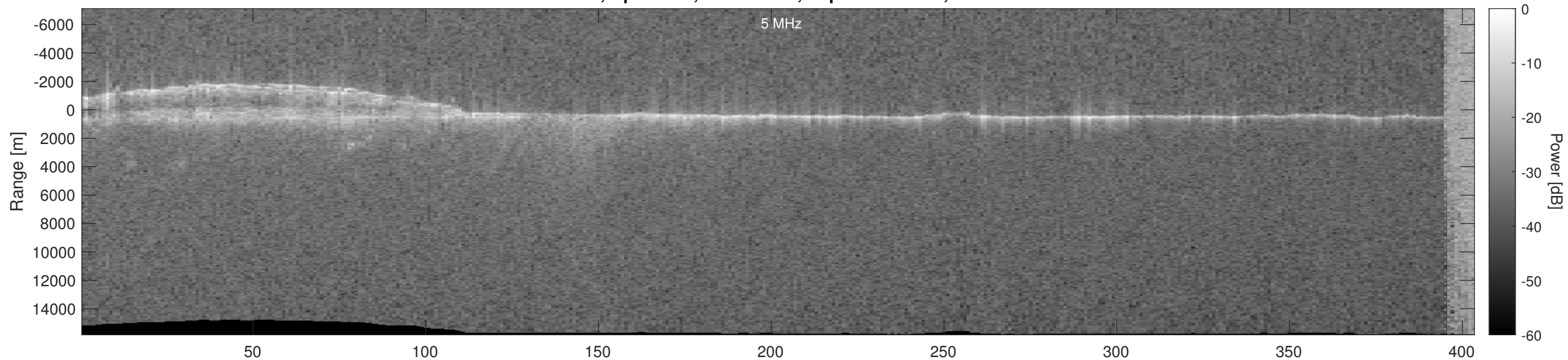
Orbit 5352, Optimized, No Window, Depth-Corrected, Channel 2
