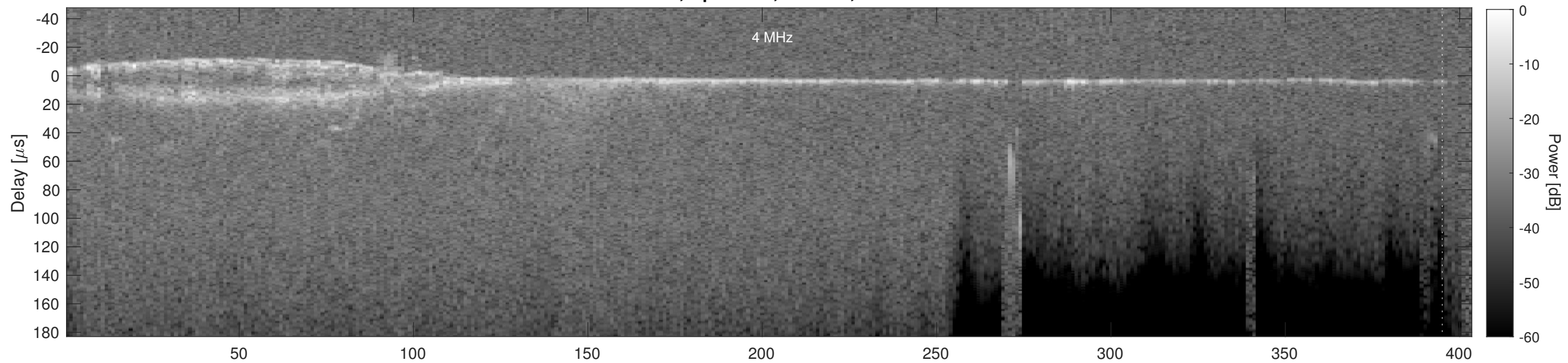
Orbit 5352, Cluttergram
