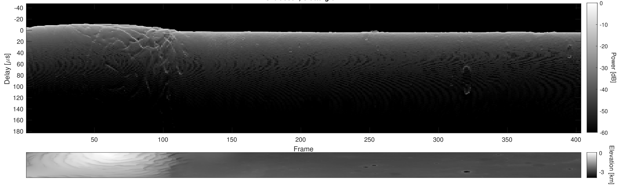
Orbit 5352, Cluttergram
