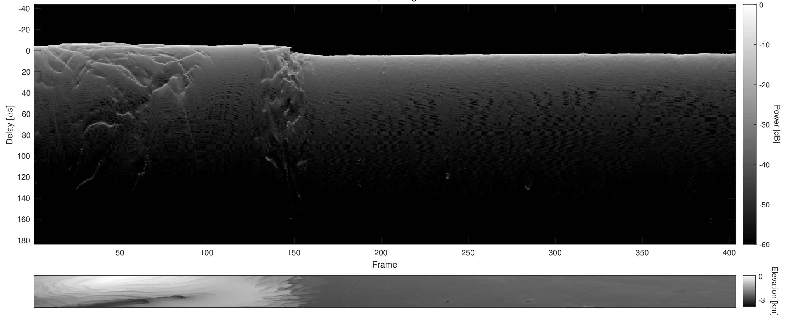
Orbit 5353, Cluttergram
