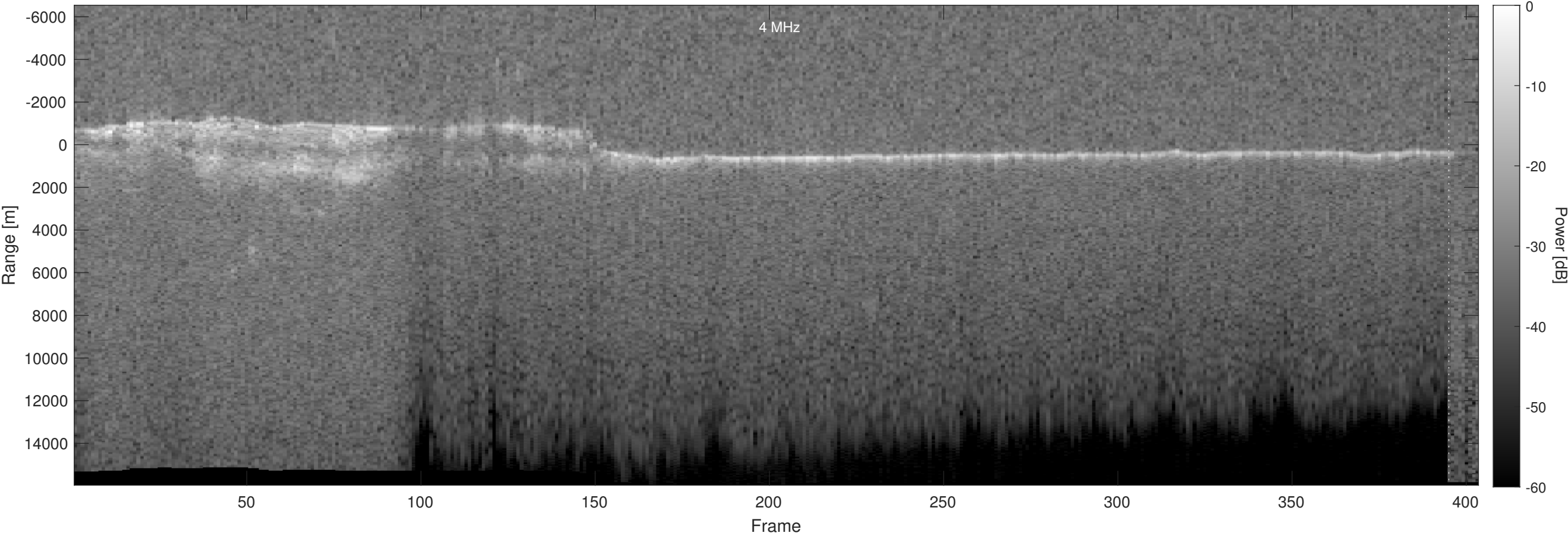
Orbit 5353, Optimized, No Window, Depth-Corrected, Channel 2
