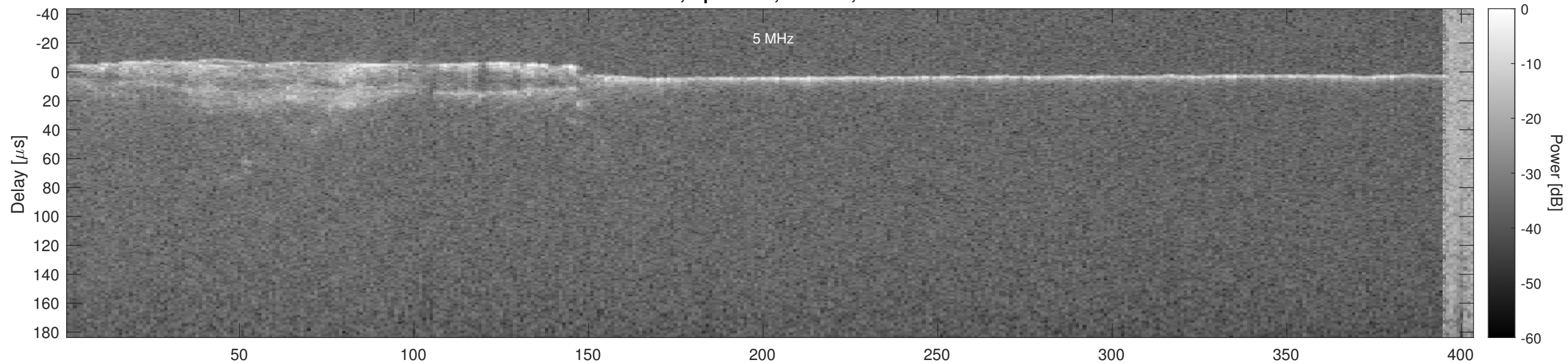
Orbit 5353, Optimized, Window, Channel 2
