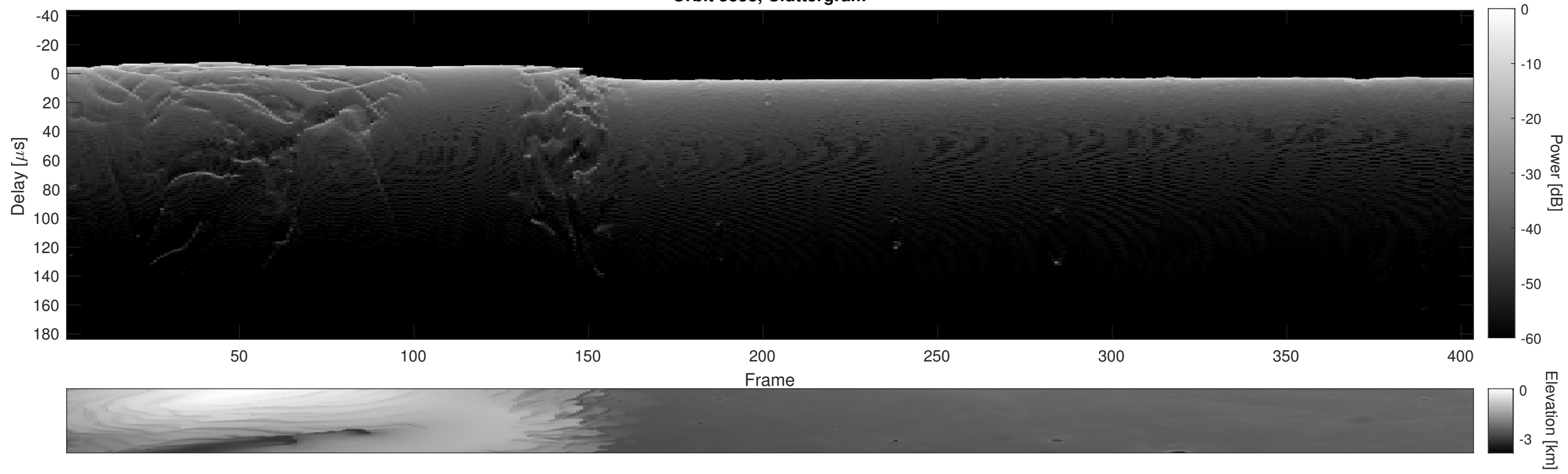
Orbit 5353, Cluttergram
