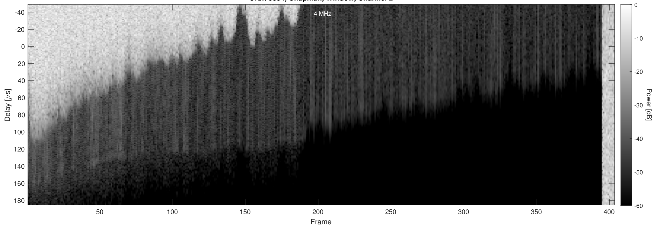
Orbit 5354, Chapman, Window, Channel 2
