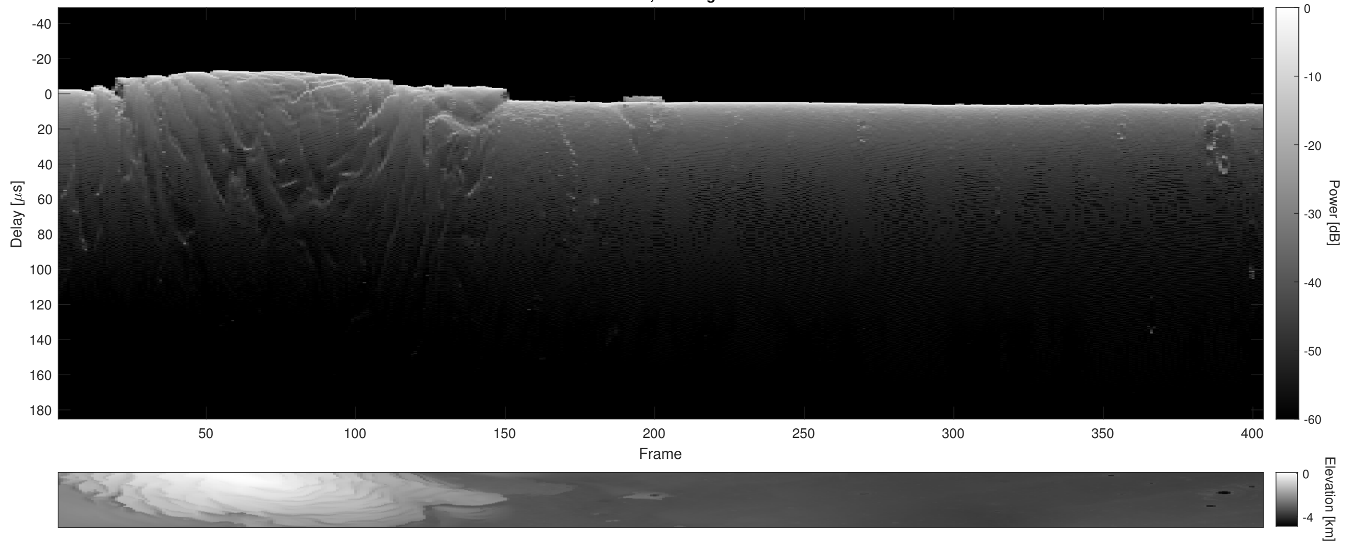
Orbit 5354, Cluttergram
