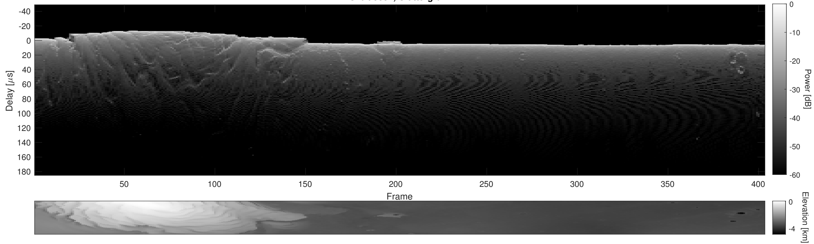
Orbit 5354, Cluttergram
