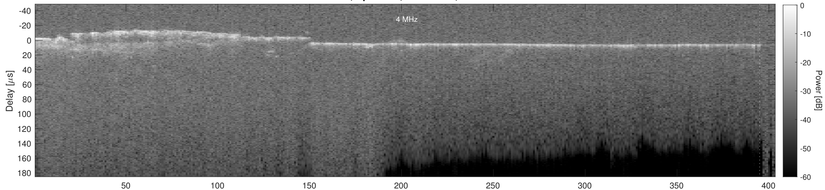
Orbit 5354, Cluttergram
