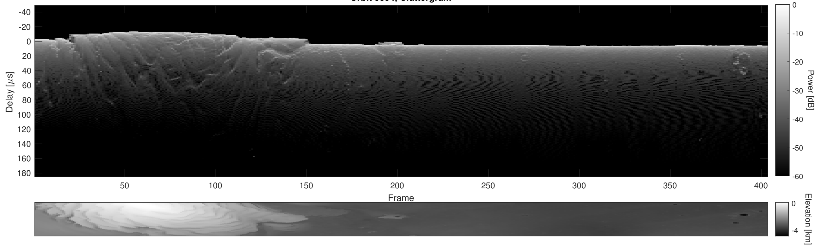
Orbit 5354, Cluttergram
