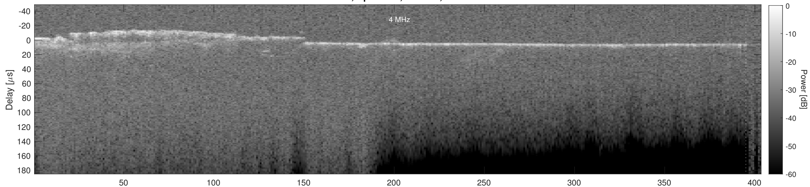
Orbit 5354, Cluttergram
