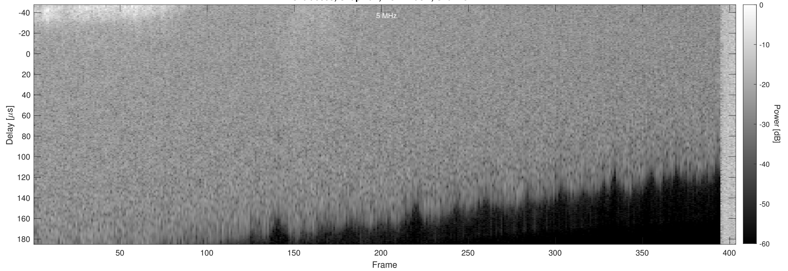
Orbit 5355, Chapman, No Window, Channel 2
