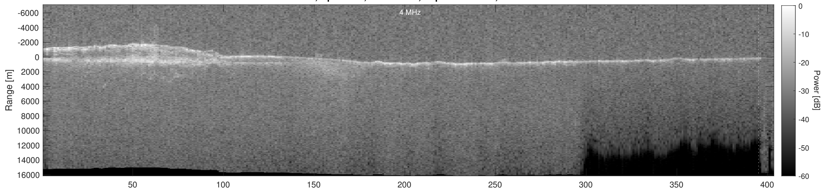
Orbit 5355, Depth-Corrected Cluttergram
