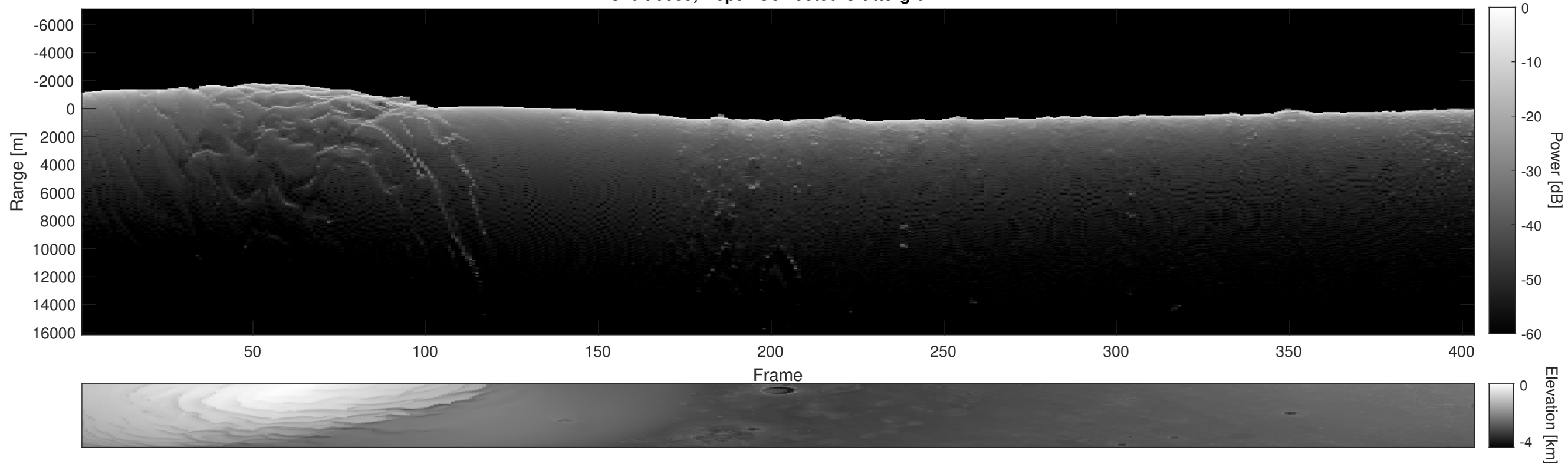
Orbit 5355, Depth-Corrected Cluttergram
