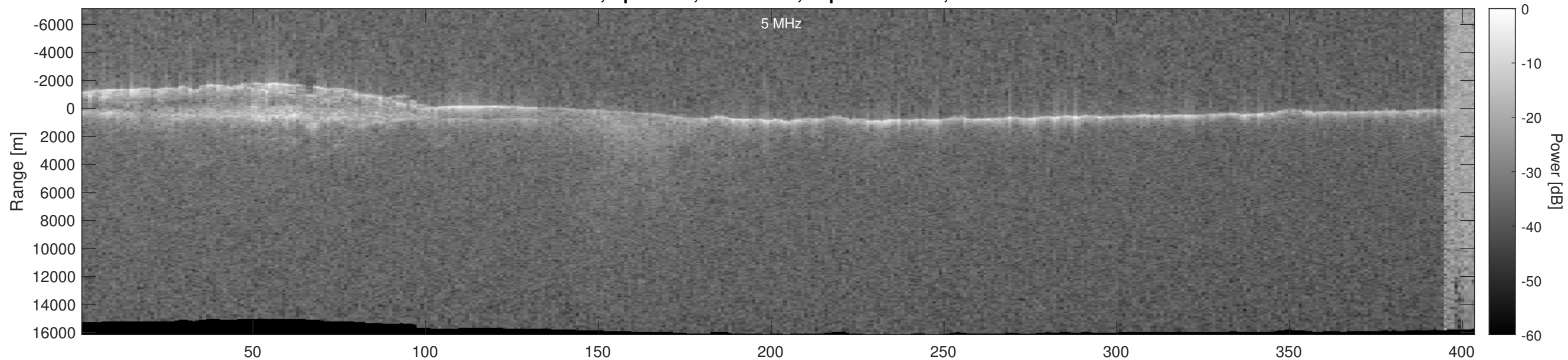
Orbit 5355, Optimized, No Window, Depth-Corrected, Channel 2
