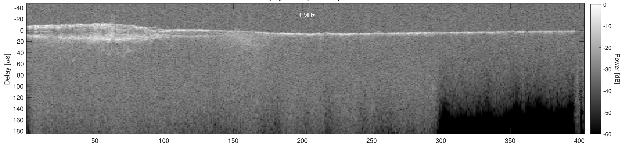
Orbit 5355, Cluttergram
