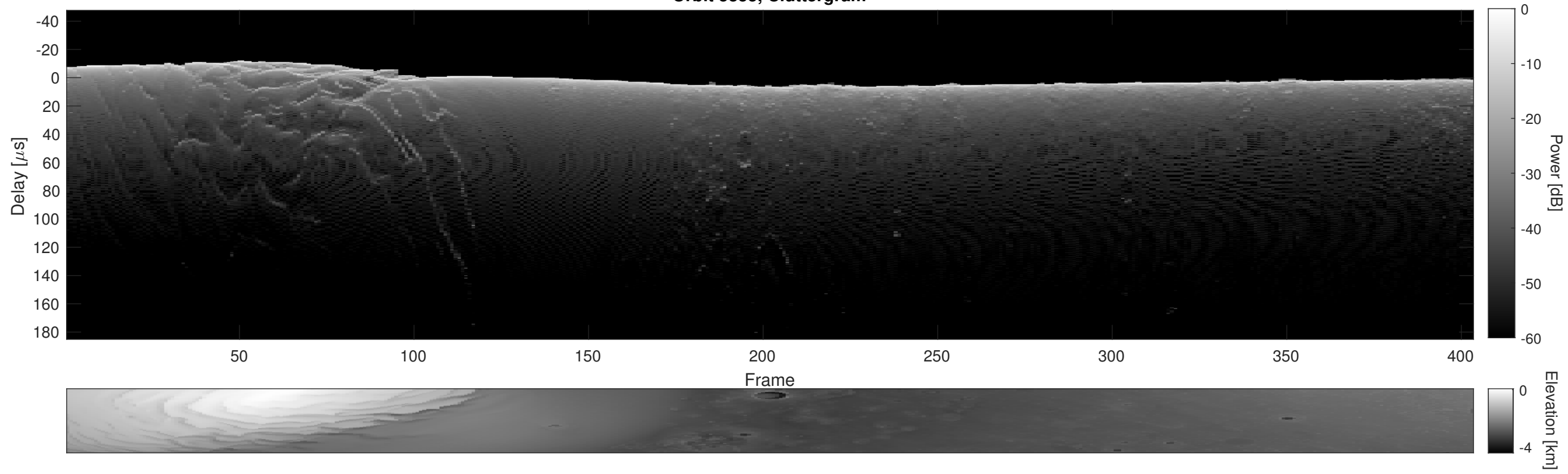
Orbit 5355, Cluttergram
