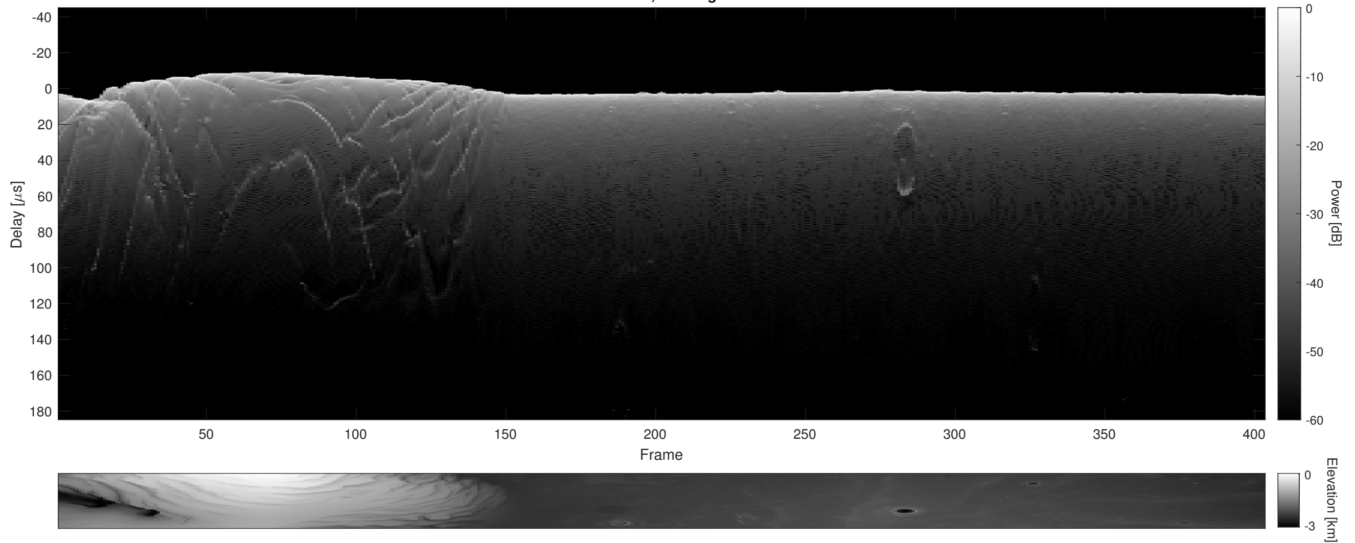
Orbit 5356, Cluttergram
