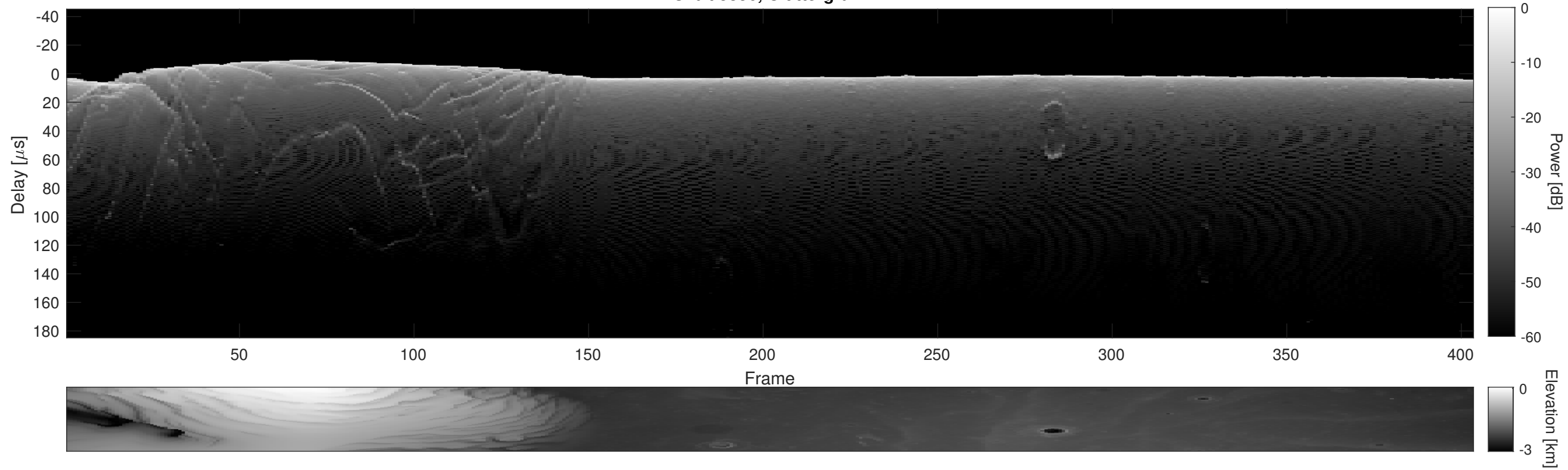
Orbit 5356, Cluttergram
