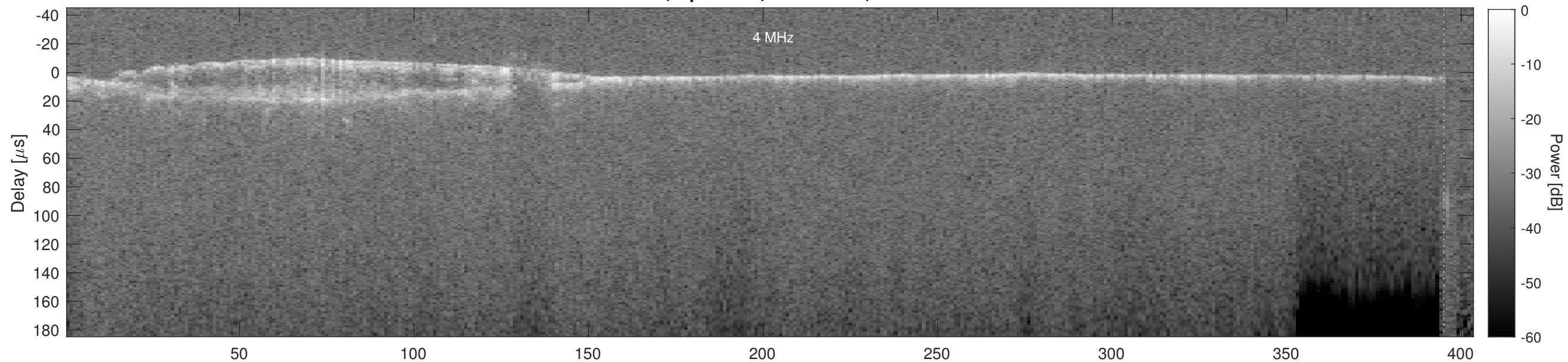
Orbit 5356, Cluttergram
