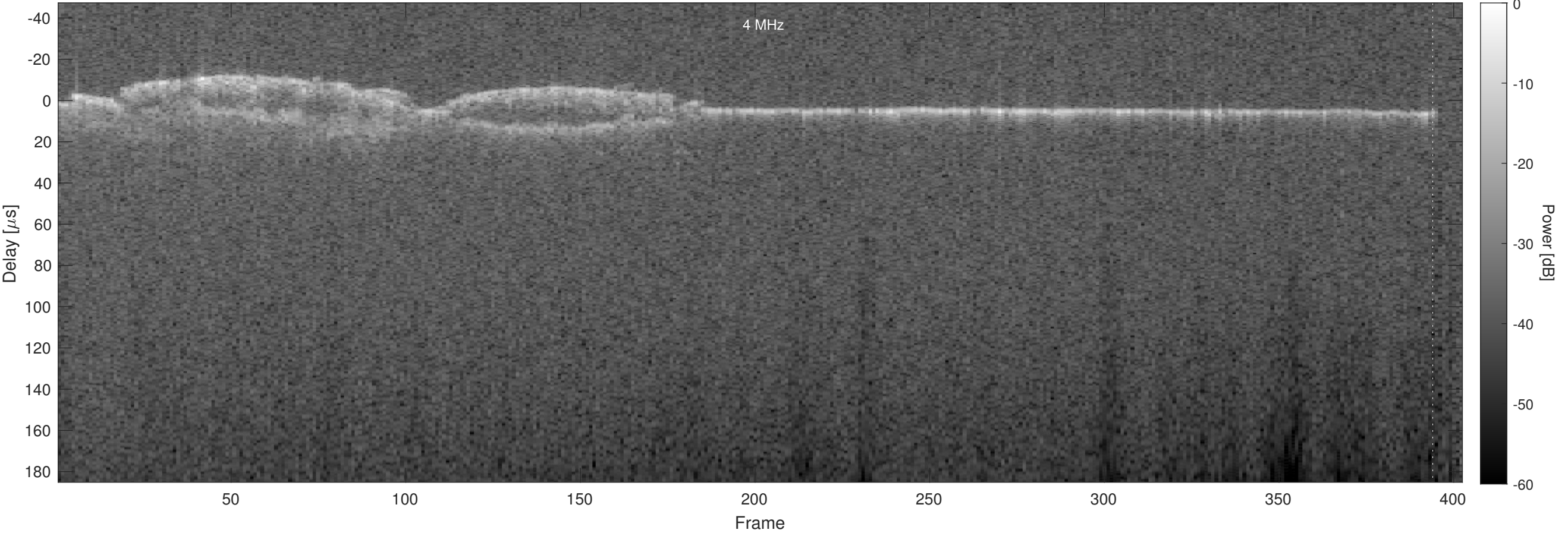
Orbit 5357, Optimized, No Window, Channel 2
