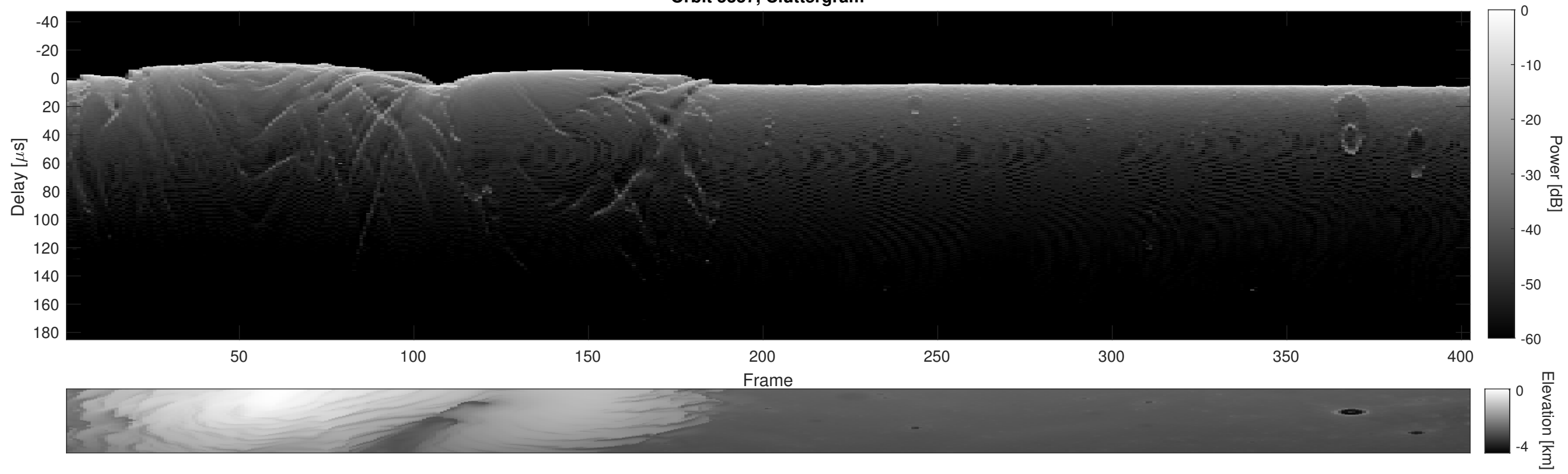
Orbit 5357, Cluttergram
