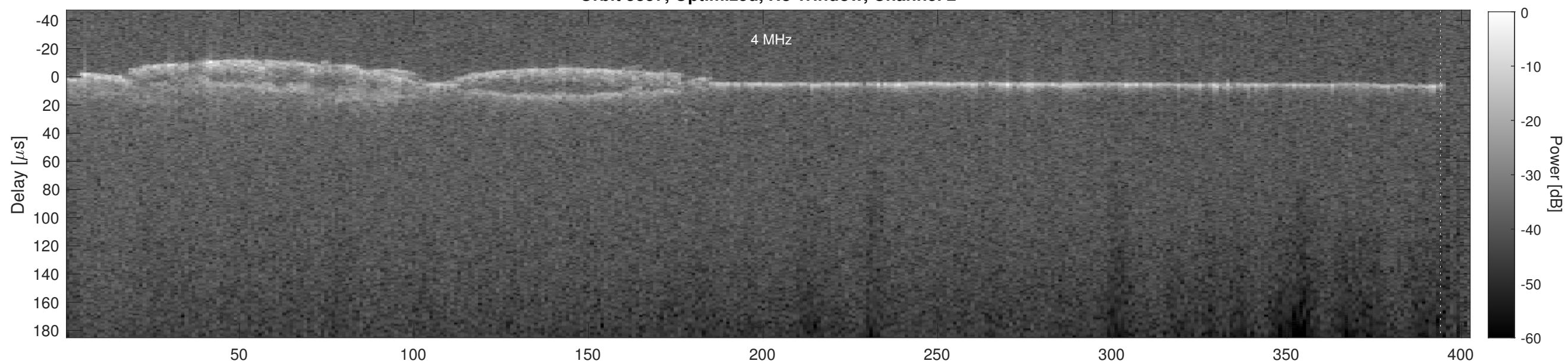
Orbit 5357, Cluttergram
