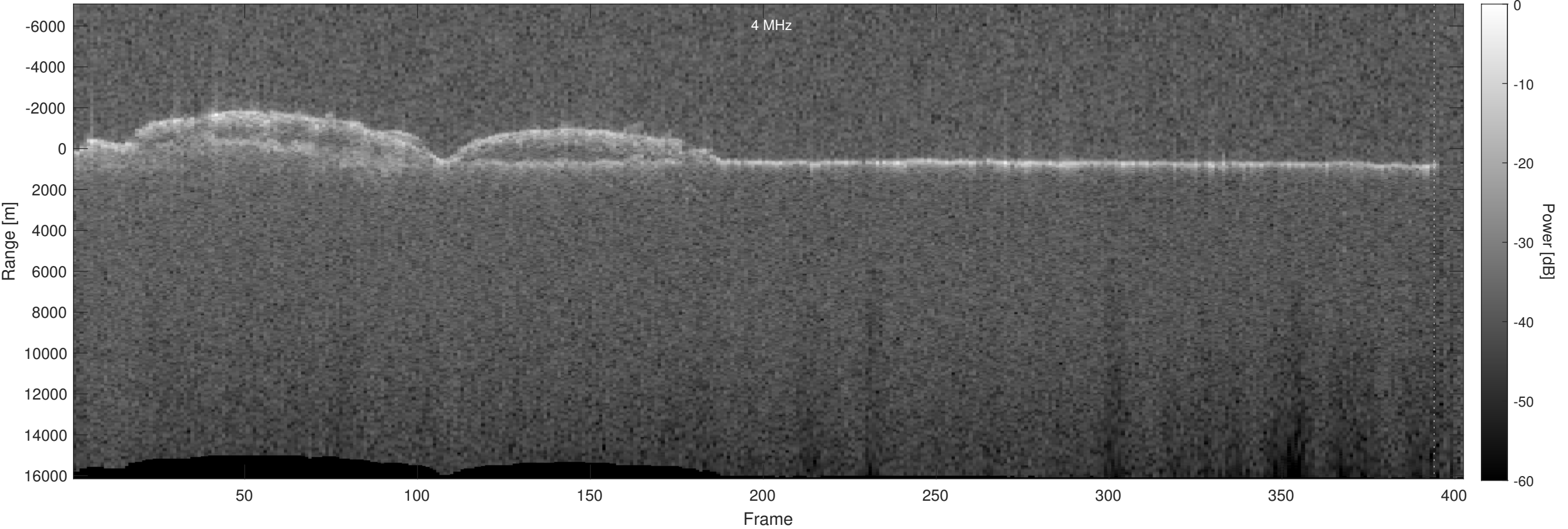
Orbit 5357, Optimized, No Window, Depth-Corrected, Channel 2
