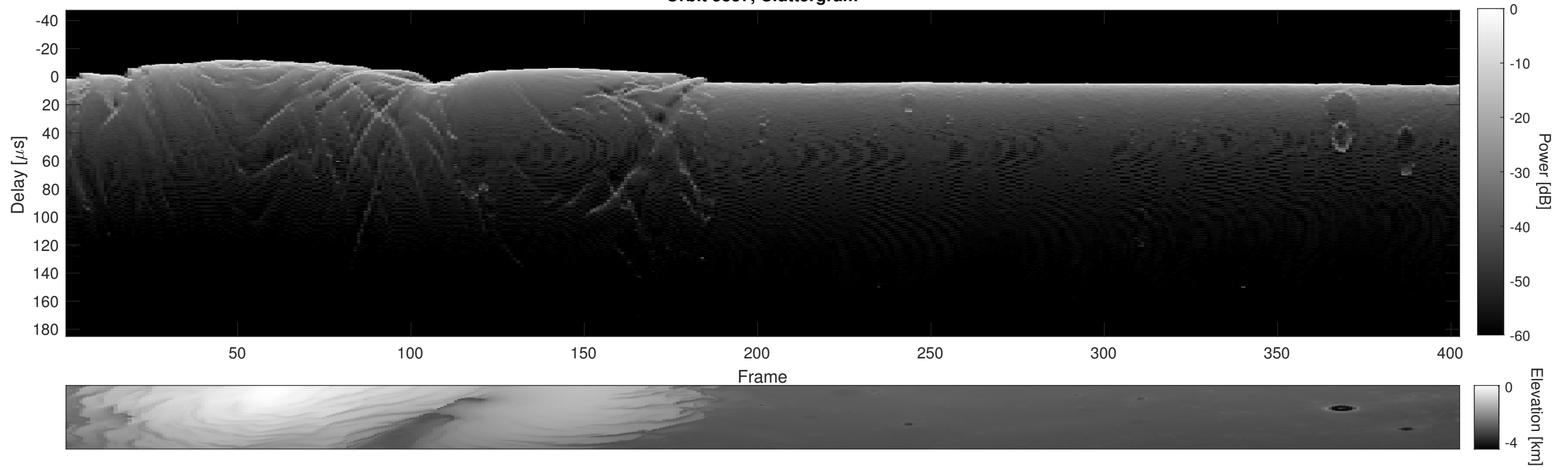
Orbit 5357, Cluttergram
