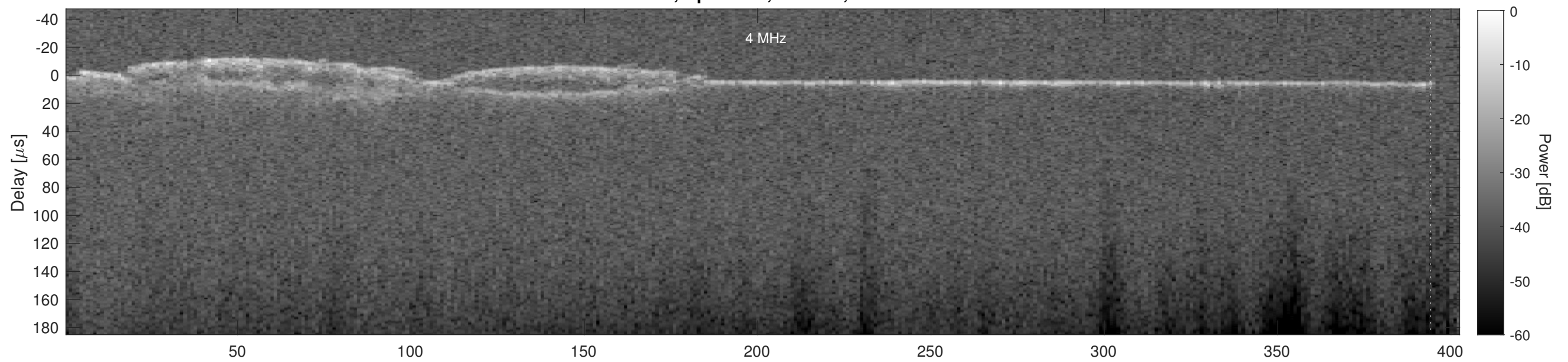
Orbit 5357, Cluttergram
