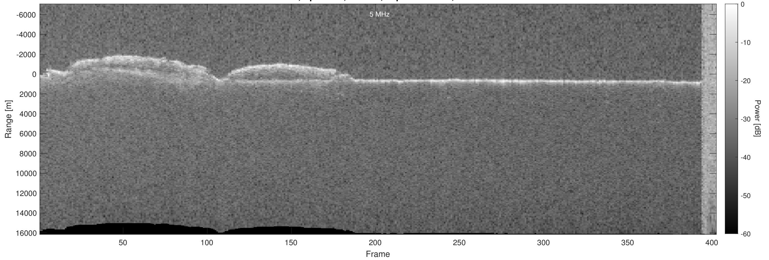
Orbit 5357, Optimized, Window, Depth-Corrected, Channel 2
