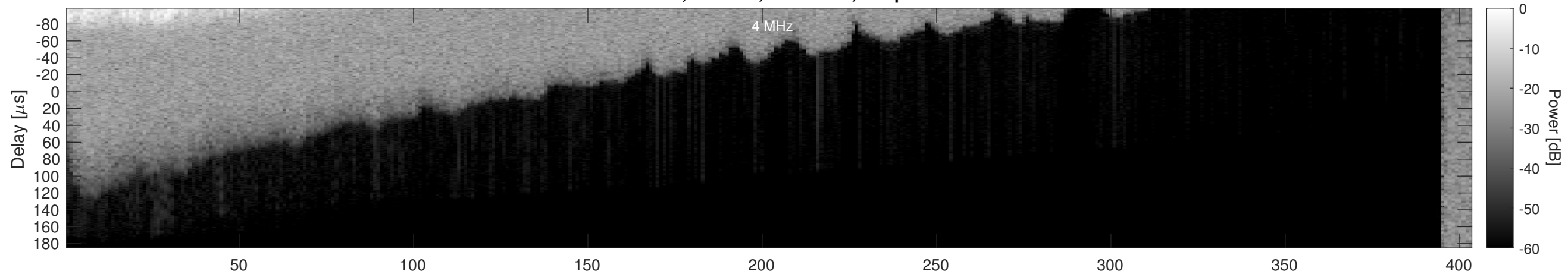
Orbit 5358, Window, Channel 2, Optimized
