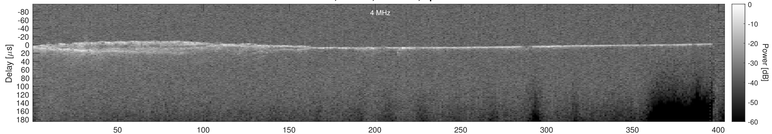
Orbit 5358, Cluttergram
