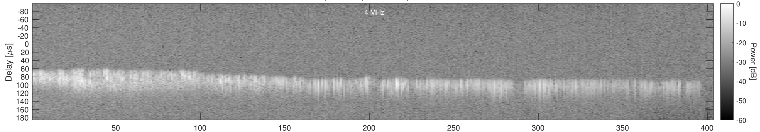
Orbit 5358, Window, Channel 2, Chapman
