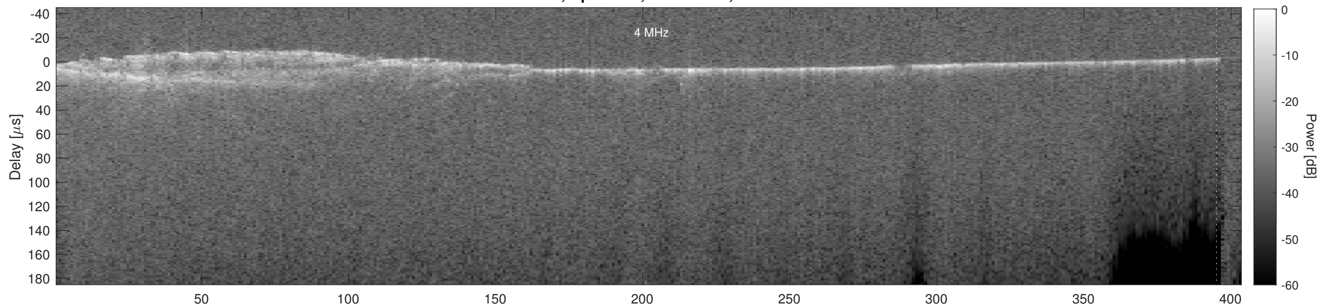
Orbit 5358, Cluttergram
