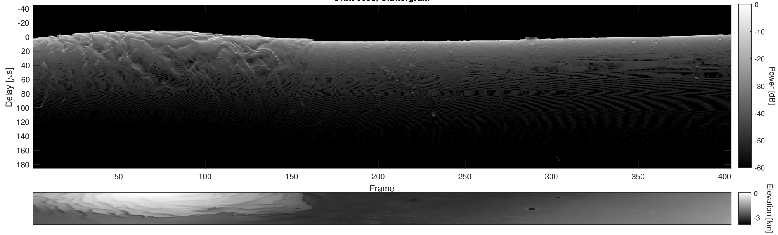
Orbit 5358, Cluttergram
