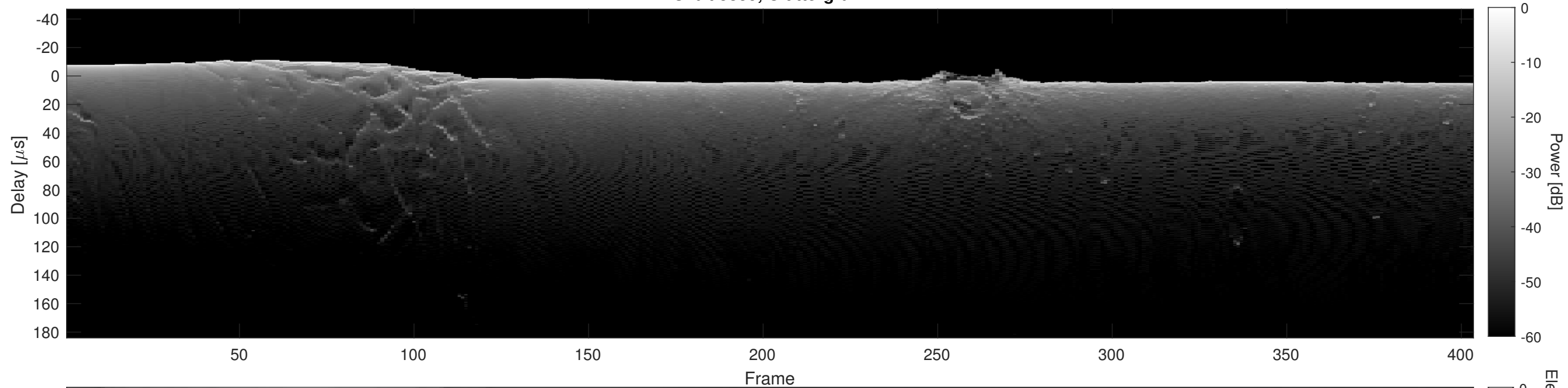
Orbit 5359, Cluttergram
