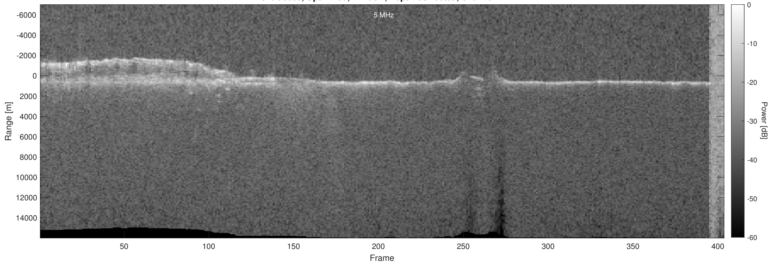
Orbit 5359, Optimized, Window, Depth-Corrected, Channel 2
