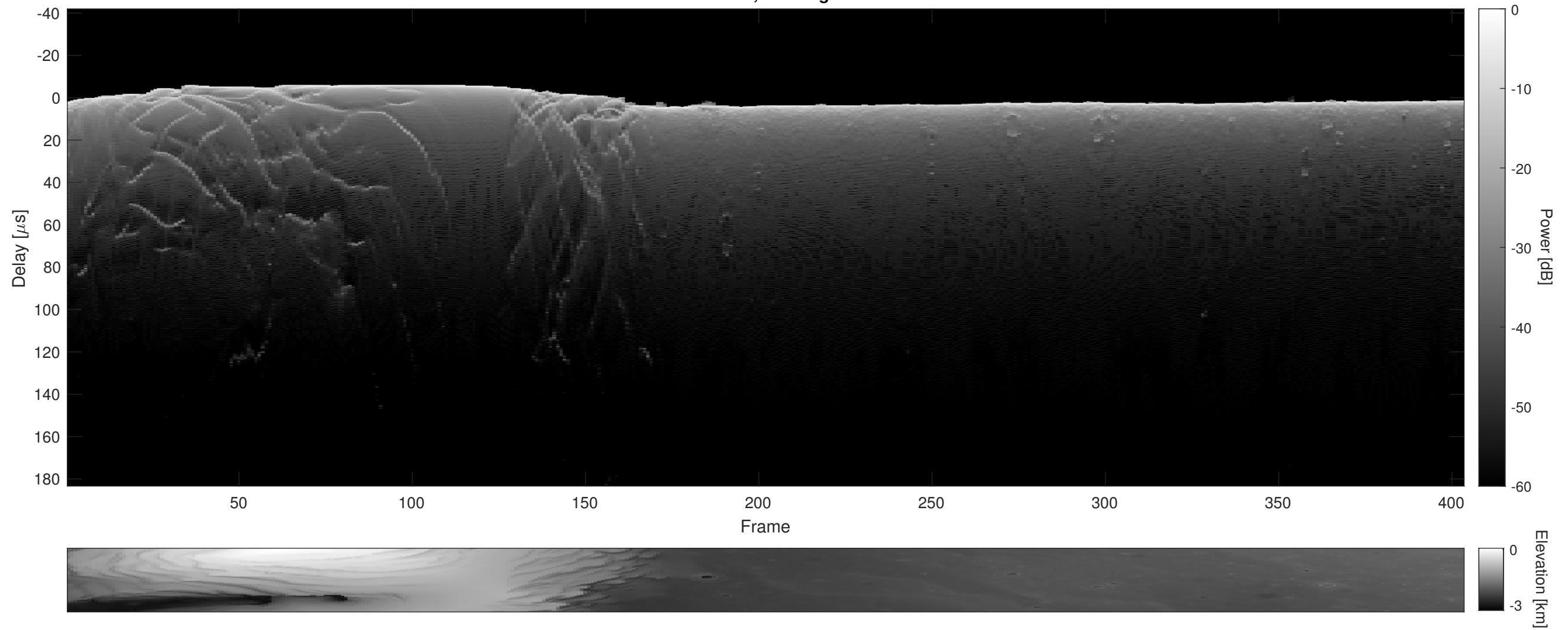
Orbit 5360, Cluttergram
